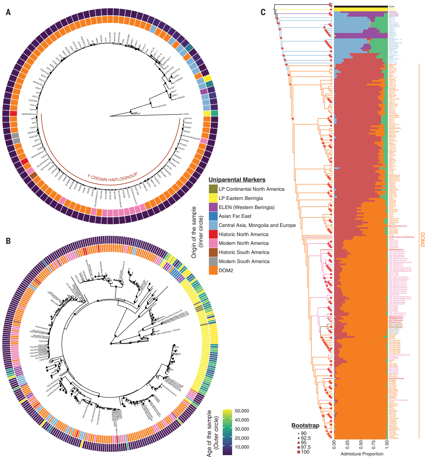
Fig. 2. Phylogenetic affinities. (A) Y-chromosomal maximum-likelihood tree ( N = 110 ; 5244 nucleotide transitions). (B) Mitochondrial maximum-likelihood tree ( N = 340 ; 16,406 base pairs). (C) Neighbor-joining tree based on ~7.5 million nucleotide transitions ( N = 241 ; left), and the corresponding genetic ancestry profiles (right). The ancestry proportions for K = 7 genetic components were
