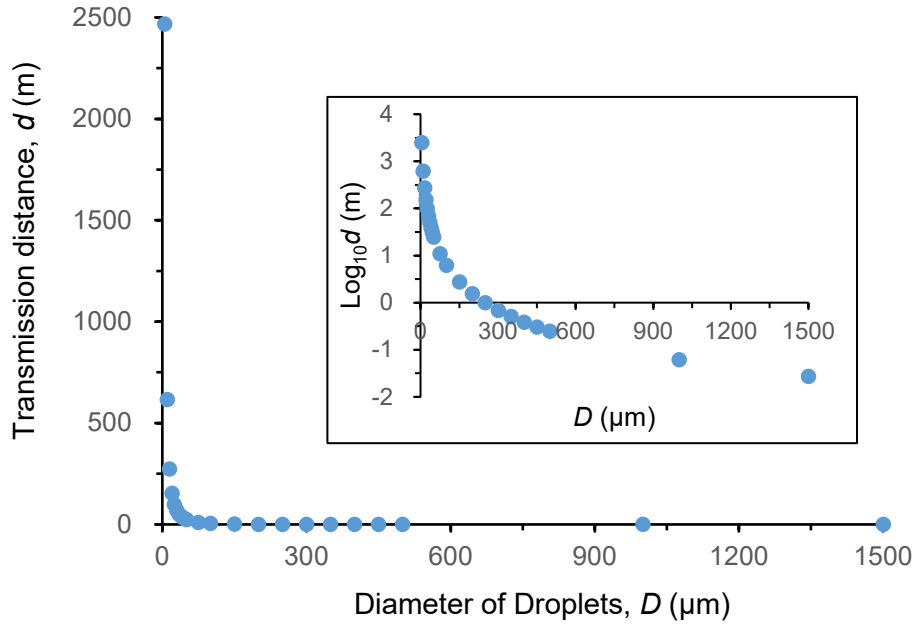
Figure 3 The transmission distance of droplets with different sizes
