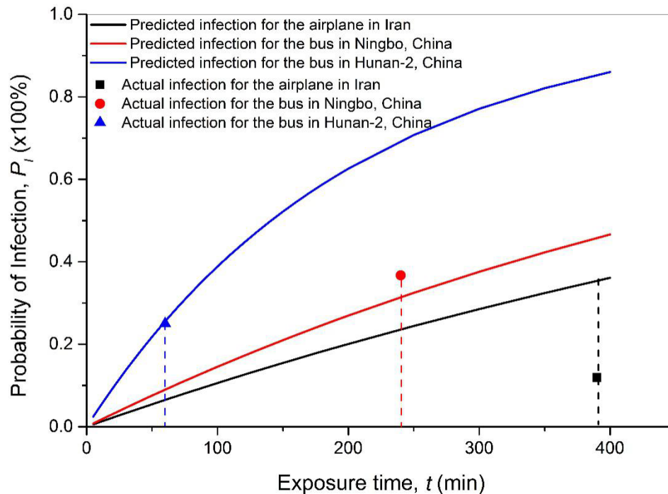
Figure 6 The predicted and actual probability of infection in existing cases
