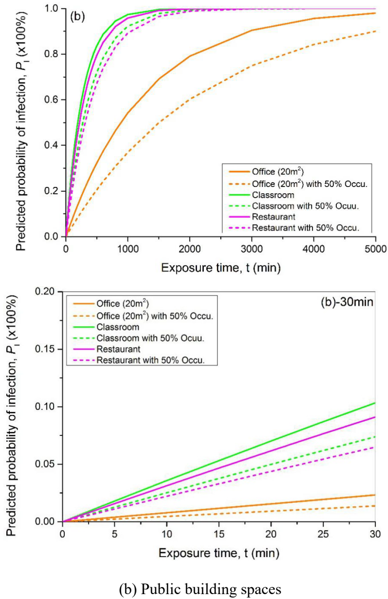
Figure 7 Predicted probability of infection for different scenarios
