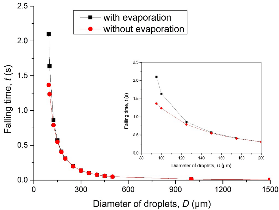
Figure 5 The falling time of droplets of different sizes with and without evaporation
