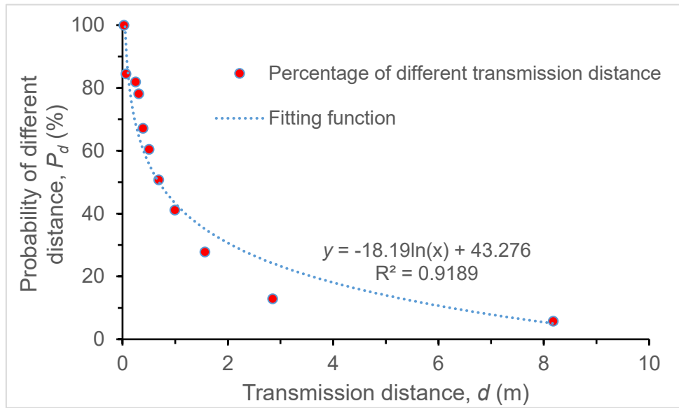
Figure 4 The relationship between droplet transmission distance and its exposure probability
