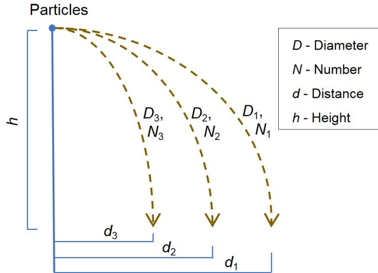
Figure 2 Transmissions of particles with different sizes
