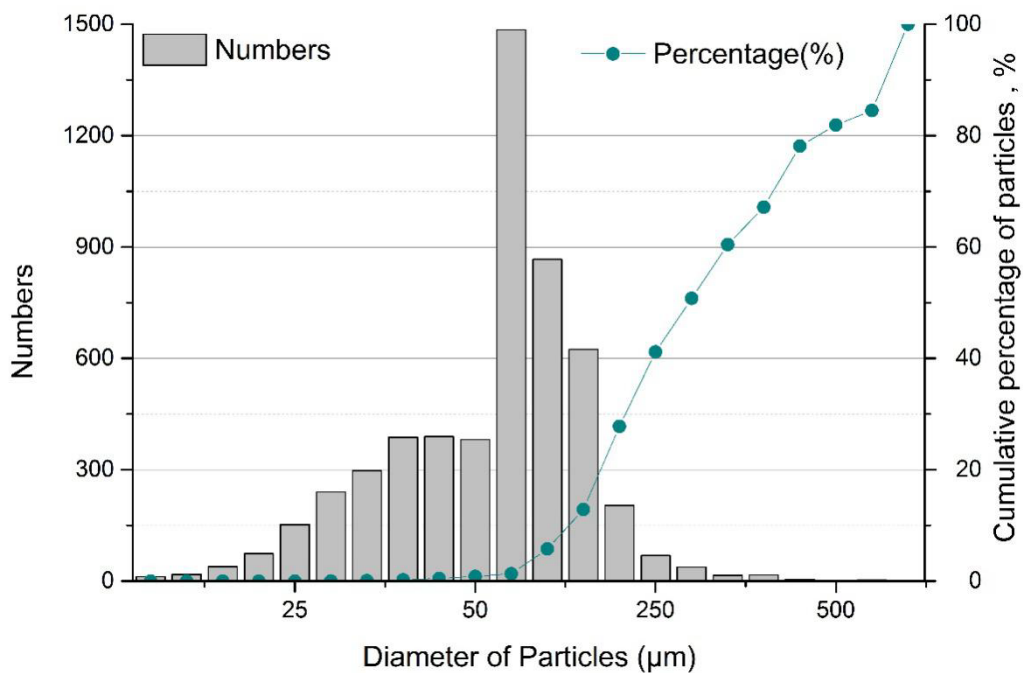
Figure 1 Sizes, numbers and cumulative mass percentages of respiratory droplets (Xie et al. 2009)
