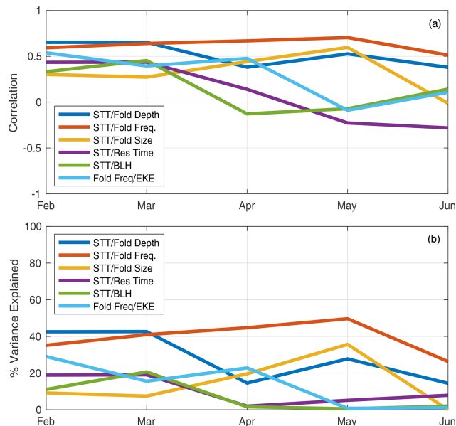
Figure 7. (a) Time series of the correlation ( r ) of monthly mean STT-PBL with various tropopause fold characteristics, residence time of PC1 \pm 5 , mean PBL height, and mean EKE. Panel (b) shows the corresponding percent variance ( r^2 ) explained by each relationship.
