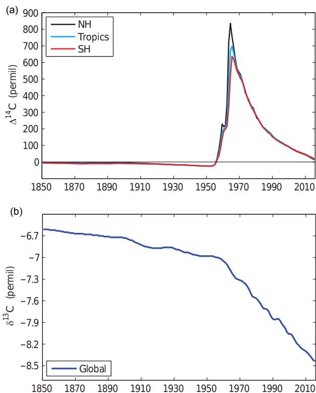
Figure 1. Historical atmospheric forcing datasets for \Delta^{14}\text{C} in CO 2 (a) and \delta^{13}\text{C} in CO 2 (b) compiled for CMIP6. Annual mean values of \Delta^{14}\text{C} are provided for three zonal bands representing the Northern Hemisphere (30–90° N), the tropics (30° S–30° N) and the Southern Hemisphere (30–90° S). Annual mean, global mean values are provided for \delta^{13}\text{C} . Tabulated data are provided in Table S1.
