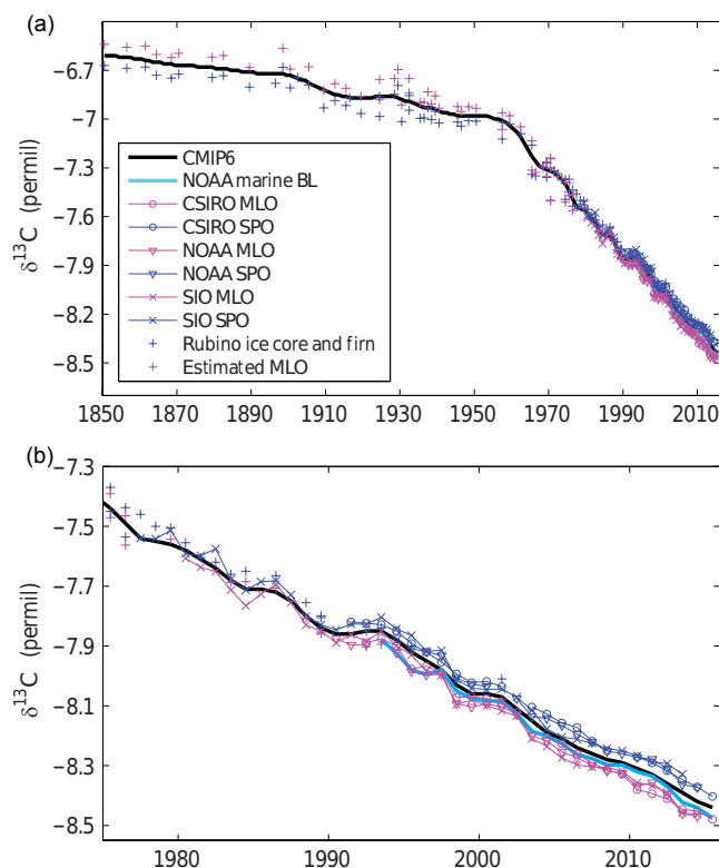
Figure 3. Observations of \delta^{13}\text{C} and the \delta^{13}\text{C} atmospheric forcing data for CMIP6 over the full time period 1850–2015 (a) and over the recent period 1975–2015 (b). The \delta^{13}\text{C} atmospheric forcing data for CMIP6 are shown in black, as in Fig. 1. Data from SPO and ice core and firn samples are shown in blue, and data from MLO and estimated data for MLO based on ice core and firn samples and the regression from Keeling et al. (2011) are shown in purple. Measurements conducted at different laboratories are shown with different symbols. Data from NOAA and SIO have been adjusted with their average laboratory offset from CSIRO. The global mean \delta^{13}\text{C} estimated by NOAA based on a larger network of flask sampling stations over 1993–2015 is shown in light blue (NOAA Marine Boundary Layer).
