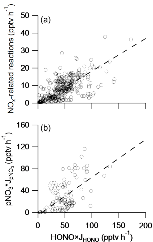
Figure 5. Correlation analysis of the main HONO sink (“HONO \times J_{\text{HONO}} ”) with the contribution from \text{NO}_x -related reactions (a) and with the contribution from particulate nitrate photolysis, p\text{NO}_3 \times J_{p\text{NO}_3} (b) in the southeastern US during the NOMADSS 2013 summer study. The line represents the Deming least-squares regression (Wu and Yu, 2018) ( r^2 = 0.40 , intercept = -0.51 and slope = 0.19 for (a); r^2 = 0.34 , intercept = -5.0 and slope = 0.69 for (b)).
