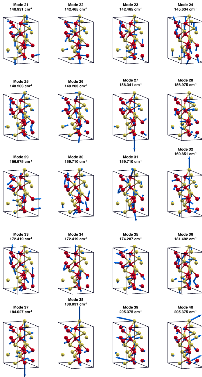
Figure 3.13: Phonon modes 21-40 of troilite. Fe and S atoms are labeled red and yellow, respectively, and the blue arrows indicate the relative amplitude and direction of the atom's movement.
