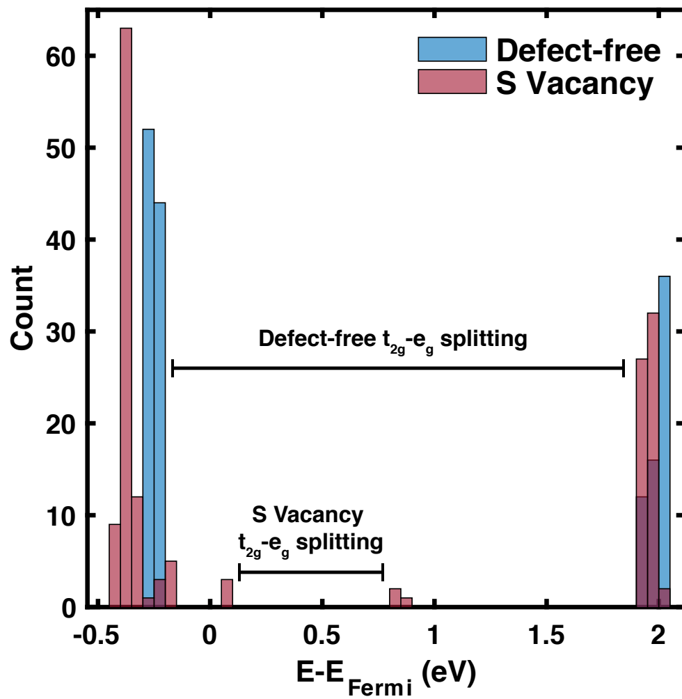
Figure 4.18: Comparison of defect-free and S deficient Fe d-orbital on-site energies. Here we clearly see the collapse of the crystal field splitting, although only six orbitals contribute to the midgap defect states. The majority of the Fe d-orbitals remain in the defect-free splitting regime.
