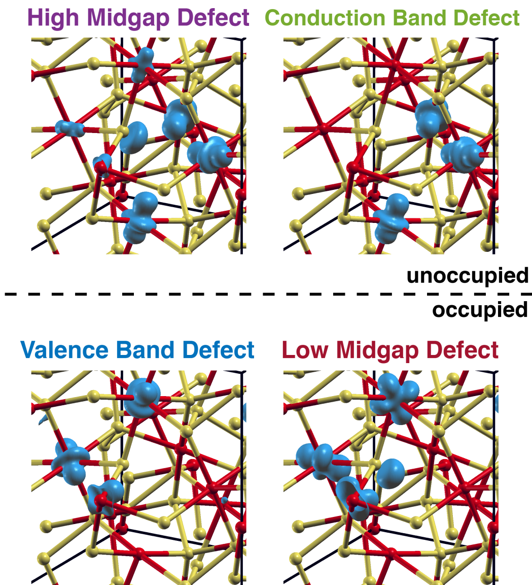
Figure 4.19: Electron density visualization of each of the four defect states in the adiabatic representation. All states are localized to the atoms surrounding the S vacancy since the charge density contours contain at least 90% of the total charge density for each state, and the defect states are color-coded to match the DOS and band structure in Figures 4.9 and ??, respectively. The occupied valence band and low midgap defect states are localized to the Fe atoms coordinated to under-coordinated S atom due to the vacancy. The unoccupied high midgap and conduction band defect states reside on the under-coordinated Fe atoms next to the S vacancy. Only the midgap states contain additional S atom character.
