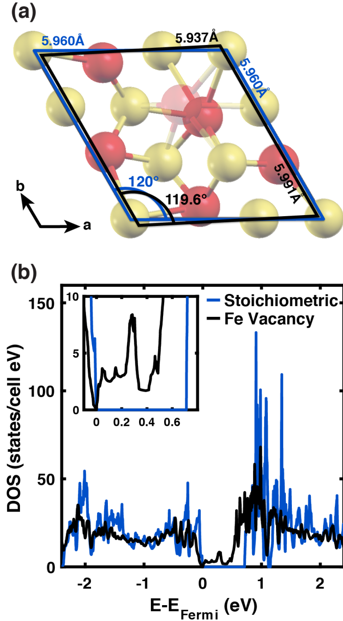
Figure 3.6: Structural and electronic deviations in FeS with and without a Fe vacancy. Panel a) shows a shift from hexagonal (blue) to monoclinic (black) geometry with the removal of an iron atom, where iron and sulfur are labeled red and yellow, respectively. The semi-transparent Fe atom denotes the vacancy in the defective structure. Spatial movements of the atoms between the defect-free and defective structure are not shown here; the atoms in the figure are included to provide context for the troilite unit cell viewed along the c-axis. The density of states for FeS with and without an iron vacancy is illustrated in b) by black and blue curves, respectively, and shows a decrease in band gap from 0.71 eV to 0 eV with the introduction of a Fe vacancy.
