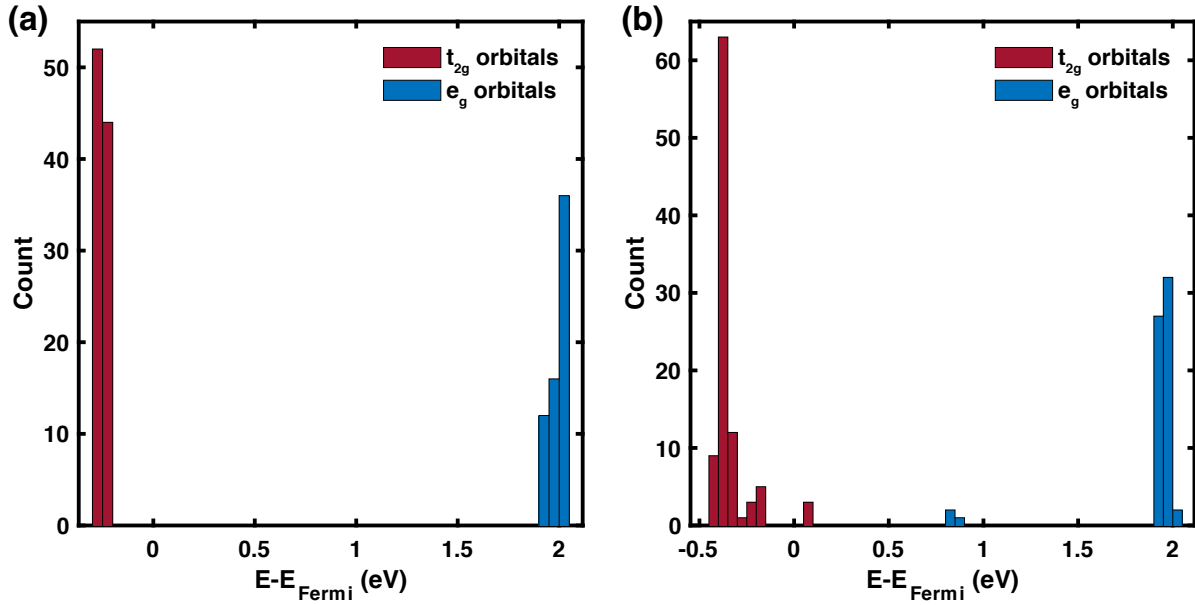
Figure 4.15: Histograms of Fe d-orbital on-site energies obtained through Wannier90 with an outer window of 0-18 eV and an inner window of 6.6-9.8 eV. Defect-free pyrite is shown in panel a) with a crystal field splitting of 2.18 eV. S deficient pyrite is shown in panel b) with a crystal field splitting of 0.73 eV due to the defect states within the octahedral splitting. In both figures, the t_{2g} orbitals have lower energy than the e_g orbitals, which we expect because of the octahedral coordination of the Fe atoms. Only six orbitals lie outside the normal splitting in panel b), confirming that the defect is spatially localized.
