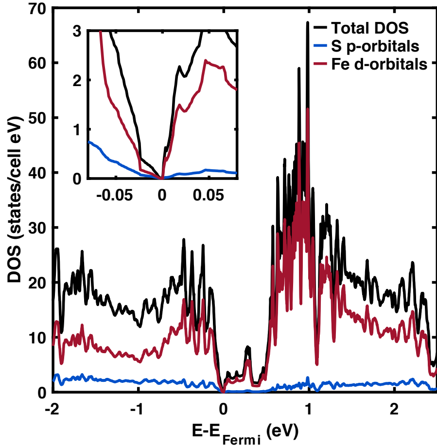
Figure 3.8: Projected density of states of iron deficient troilite. The Fe d-orbitals make up the majority of both valence and conduction bands with the S p-orbitals only contributing a small amount. All other orbitals not shown in the figure contribute insignificantly to the total DOS.
