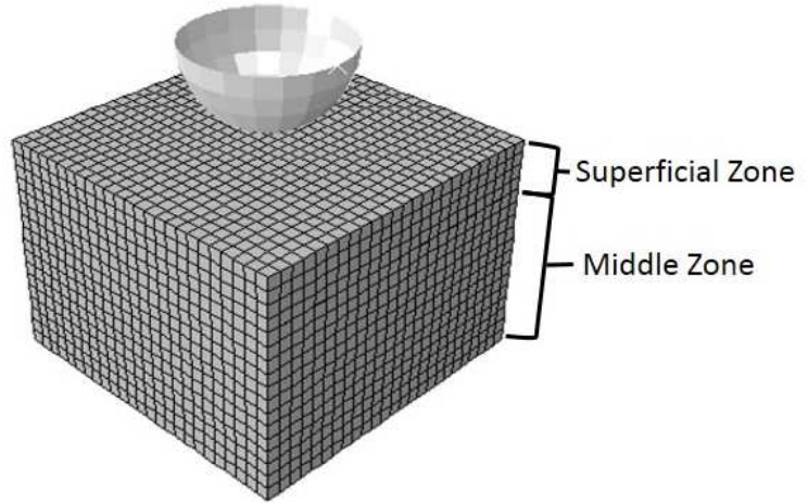
Figure 7. Finite element models showing (A) uniaxial stress in tension finite element model with dashed lines denoting the initial configuration. (B) Spherical indentation model with superficial and middle zones of articular cartilage. For spherical indentation simulations, the spherical indenter was modeled as an analytical rigid surface while the cartilage block was modeled using 10625, 8 node linear hexahedral C3D8 elements with displacements at the bottom surface constrained in all directions. The adjacent SZ and MZ of regions were constrained at the shared surface using a tied contact formulation
