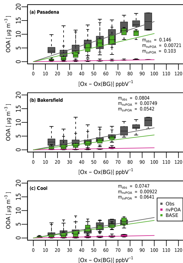
Figure 4. OOA concentrations ( \mu\text{g m}^{-3} ) at California sites as a function of the measured \text{O}_x ( \text{O}_3 + \text{NO}_2 ) concentration. A background concentration, \text{O}_x (BG), of 13.5 ppbv is assumed, consistent with Hayes et al. (2015). The boxes behind each trend indicate the 25th and 75th percentiles of the data. The whiskers extend to the 10th and 90th percentiles. The solid horizontal lines in each box identify the median, and the solid curves indicate the means of each model run. Model values are projected to \text{PM}_{10} to correspond roughly to the size cutoff of the AMS.
