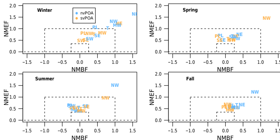
Figure 10. Regional and seasonal model performance at routine-monitoring stations for the CONUS11 simulation as a function of the normalized mean bias factor (NMBF) and normalized mean error factor (NMEF) for OC predictions. Plotted regions include the northeast (NE), Midwest (MW), southeast (SE), Plains (PL), northwest (NW), southwest (SW), and total (T) and are defined as visualized in Fig. 8.
