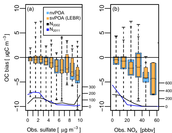
Figure 13. Organic carbon bias for CSN summer time data during 2002 and 2011 (combined) as a function of observed sulfate concentrations (a) and observed \text{NO}_x concentrations (b). The meaning of boxes and whiskers is explained in Fig. 5. Blue (2011) and black (2002) solid lines quantify the number of data points for each year as functions of the observed pollutants.
