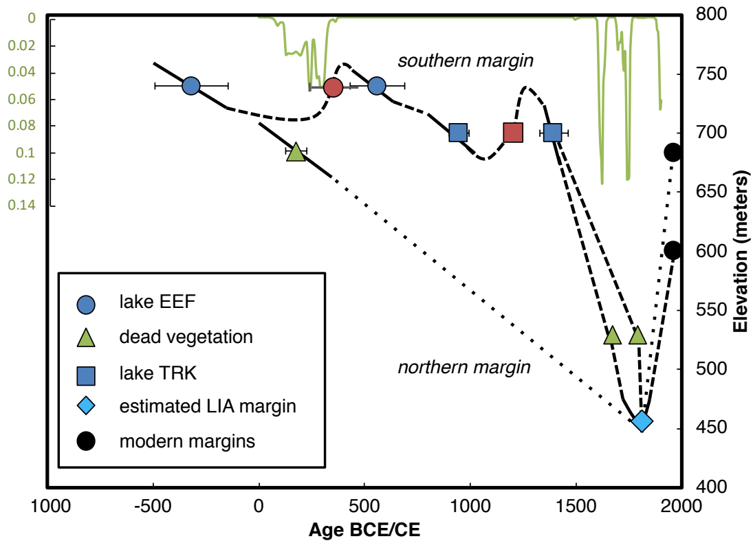
Figure 3.8: Change in ice margin elevation over the last 3 ka on the northern (dotted) and southern margins (dashed). Blue (red) indicate advance (retreats) from lake catchment thresholds. LIA margin at 1850 CE estimated from Fig. 4 and is assumed to have an error of \pm 100 meters. Error bars represent 95% confidence limit from lake age-depth models (Fig. 3.5). Cumulative PDF of southern margin emerging dead vegetation ^{14}\text{C} -dated inverted on top (see Fig. 3.5).
