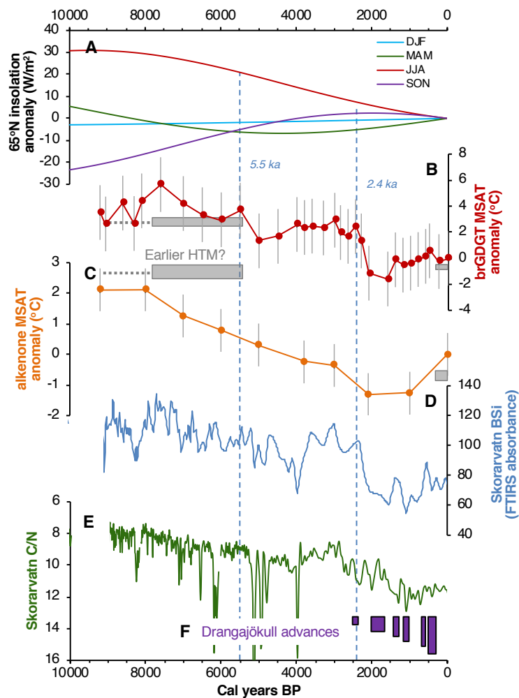
Figure 7.9: Comparisons of regional climate records to Skorarvatn's paleotemperature records. A) Seasonal insolation curves over the last 10000 years (Laskar et al., 2004), B) brGDGT MSAT anomaly from Skorarvatn (this study), C) alkenone MSAT anomaly from Skorarvatn (this study), D) biogenic silica (BSi) record from Skorarvatn (Harning et al., 2016a), E) inverted C/N record from Skorarvatn
