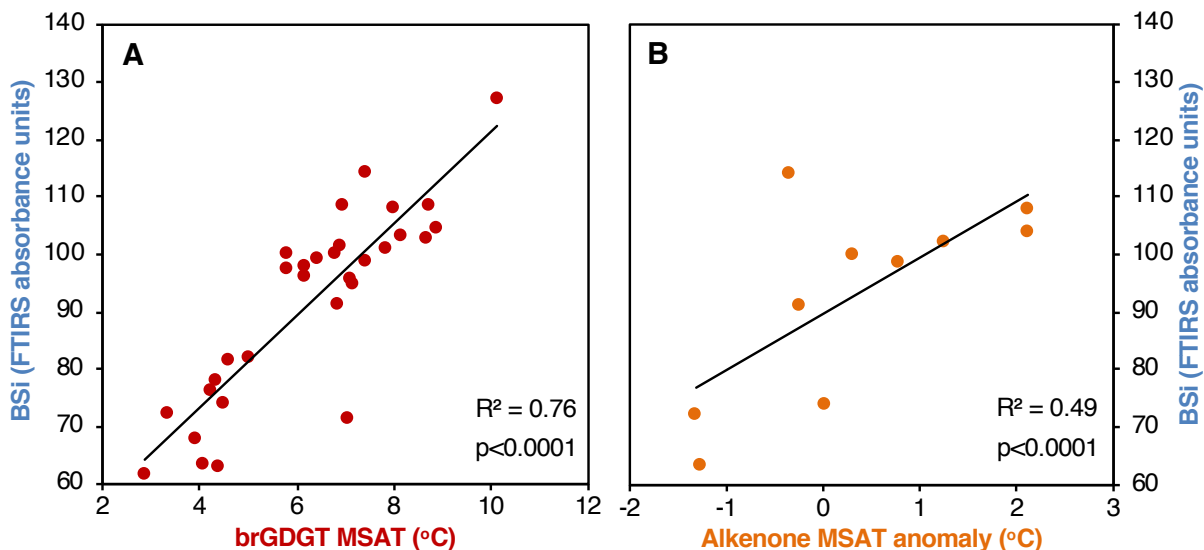
Figure 7.10: Linear regressions between biogenic silica (BSi) from Skorarvatn (Harning et al., 2016a) and A) brGDGT MSAT and B) alkenone MSAT anomaly.
