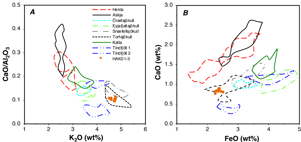
Figure 6.8: Plots of the rhyolitic component of the Settlement Layer marker tephra demonstrating origin from the Torfajökull volcanic system.
