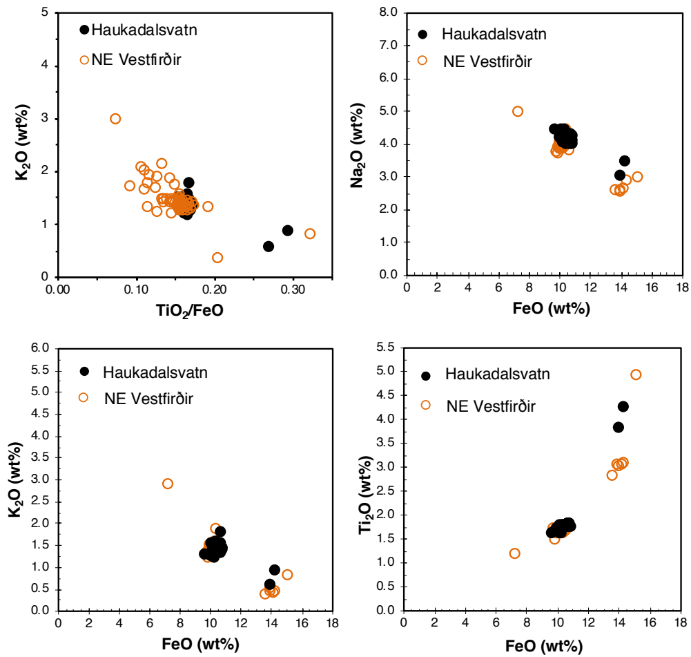
Figure S6.8: Bi-elemental plot comparisons demonstrating the correlation of the Hekla 4 marker tephra in Haukadalsvatn (n=36) to the tephra layers found in Northwest Iceland lakes (n=37, Harning et al., 2018b).
