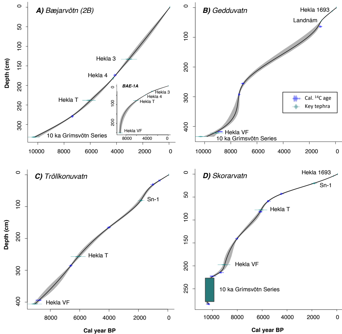
Figure 5.9: CLAM age models for A) Bæjarvötn 2B and 1A (inset), B) Gedduvatn, C) Tröllkonuvatn and D) Skorarvatn based on calibrated ^{14}\text{C} ages (blue) and key tephras of known age (green). Gray shaded areas denote the 95% confidence limit. Detailed ^{14}\text{C} information provided in Table 5.1.
