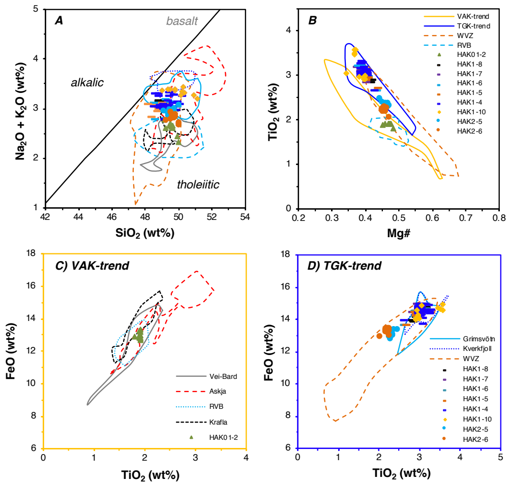
Figure 6.4: Examples of tholeiitic basalt tephra discrimination from Haukadalsvatn. Panel B enables further discrimination of tephra based on their affinity to either the VAK (Veidivötn, Askja, Krafla) volcanic systems (C) or the TGK (Thordarhyrna, Grímsvötn, Kverkfjöll) volcanic systems (D). Mg\# = (MgO_{wt\%}/40.3)/((FeO_{wt\%}/71.8)+(MgO_{wt\%}/40.3)) .
