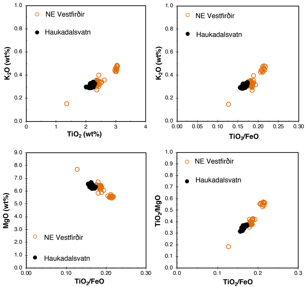
Figure S6.5: Bi-elemental plot comparisons demonstrating the correlation of the Grímsvötn BP-1 marker tephra in Haukadalsvatn (n=12) to the tephra layers found in Northwest Iceland lakes (n=40, Harning et al., 2018b).
