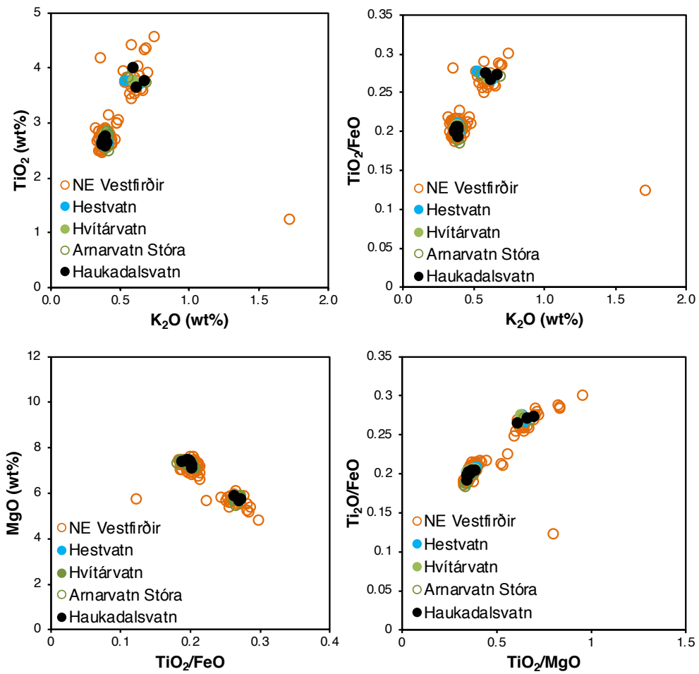
Figure S6.7: Bi-elemental plot comparisons demonstrating the correlation of the Hekla T marker tephra in Haukadalsvatn (n=12) to the tephra layers found in Northwest Iceland lakes (Harning et al., 2018b), Hestvatn (n=11, Jóhannsdóttir, 2007), Hvítárvatn (n=11, Jóhannsdóttir, 2007) and Arnarvatn Stóra (n=15, Gunnarson, 2017).
