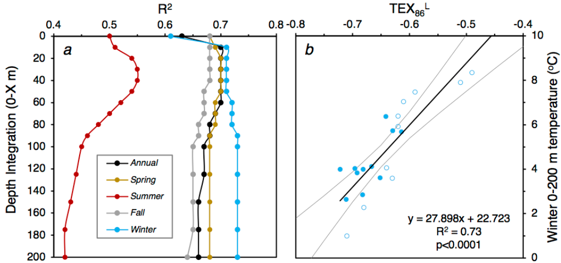
Figure 8.4: Regression analysis summary of surface sediment GDGT calibration. A) Correlation coefficient ( R^2 ) of the 21 surface sediment TEX_{86}^L values against seasonal and annual temperature depth integrations. B) Calibration of Icelandic marine surface sediment TEX_{86}^L values against winter 0-200 m temperature, where gray lines denote the 95% confidence envelope. Surface sediment data shown as closed circles (this study) and open circles (Rodrigo-Gámiz et al., 2015).
