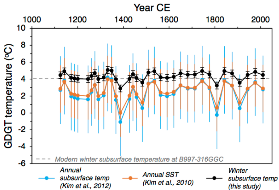
Figure 8.5: Comparison of the available \text{TEX}_{86}^L temperature calibrations on the B997-316 GGC sediment record. Icelandic winter subsurface temperature (this study), annual SST (Kim et al., 2010) and annual subsurface temperature (Kim et al., 2012). Modern winter subsurface temperature at the B997-316 GGC site marked with gray dashed line. Note: the standard error of the winter subsurface temperature ( \pm 0.4^\circ\text{C} ) is shown, but hardly visible given the diameter of the data points.
