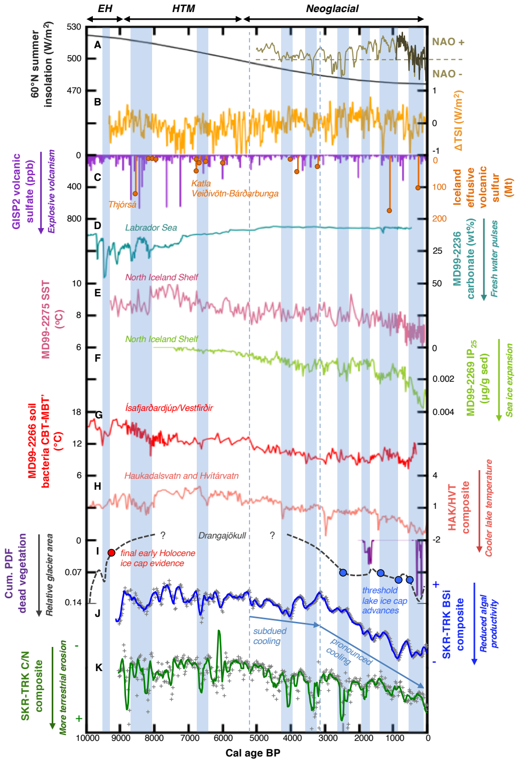
Figure 4.7: Comparison of potential climate forcings to northern North Atlantic, Icelandic and Vestfirðir climate records. A) 60°N summer insolation ( \text{W/m}^2 , Berger and Loutre, 1991), and NAO variability reconstructed from SW Greenland (light brown, Olsen et al., 2012) and Morocco-Scotland (dark brown, Trouet et al., 2009), B) \Delta\text{TSI} derived from ice core ^{10}\text{Be} (Steiniliber et al., 2009), C) GISP2
