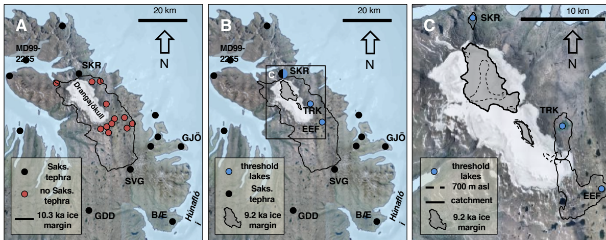
Figure 2.5: A) Estimated extent of proto-Drangajökull at 10.3 ka. Black circles mark locations of sediment cores or soil sections containing undisturbed Saksunarvatn tephra, as described by Andrews et al. (2002), Geirsdóttir et al., (2002), Principato et al. (2006) and this study. Red circles mark locations of sediments cores containing no Saksunarvatn tephra, as described by Schomacker et al. (2016), Harning et al. (2016) and this study. B) Remnant ice cap margin at 9.2 ka with relevant threshold lakes marked by blue circles. C) Close-up of remnant ice margin shown at 9.2 ka. Subglacial lake catchments and 700 m asl bedrock contour were extracted from a subglacial topographic DEM by (E. Magnússon, pers. comm.). 2005 base image courtesy of Loftmyndir ehf.
