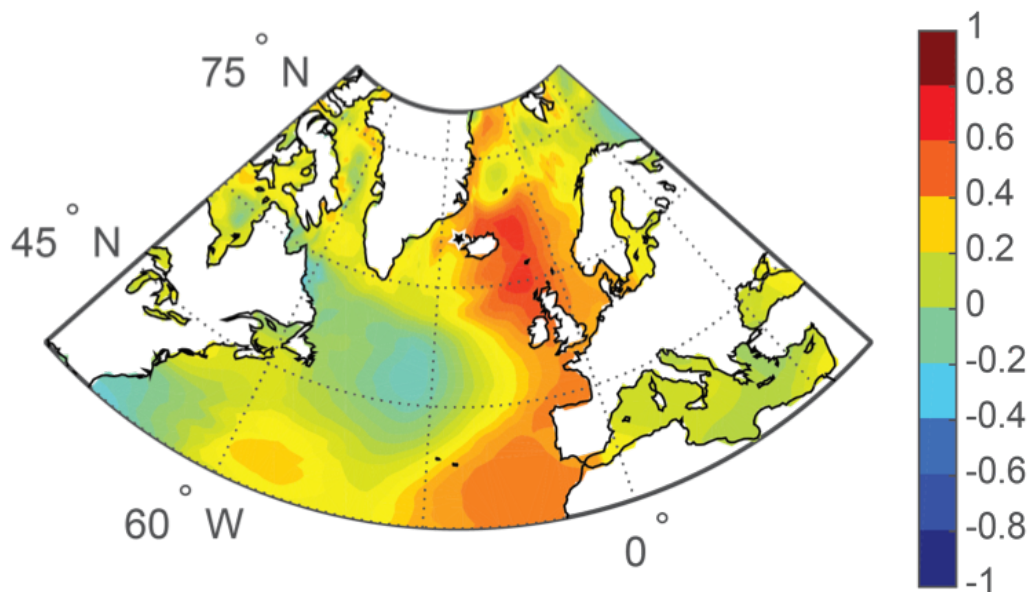
Figure 3.1: Correlation of gridded JJA SSTs to JJA surface air temperature at Drangajökull (black star). See supplemental for details on methodology.
