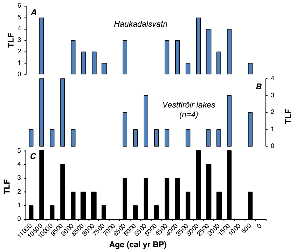
Figure 6.12: Tephra layer frequency (TLF) in 500-yr bins for A) Haukadalsvatn, West Iceland (this study), B) Vestfirðir lakes, Northwest Iceland (Harning et al., 2018b), and C) sum of Haukadalsvatn and Vestfirðir lakes.
