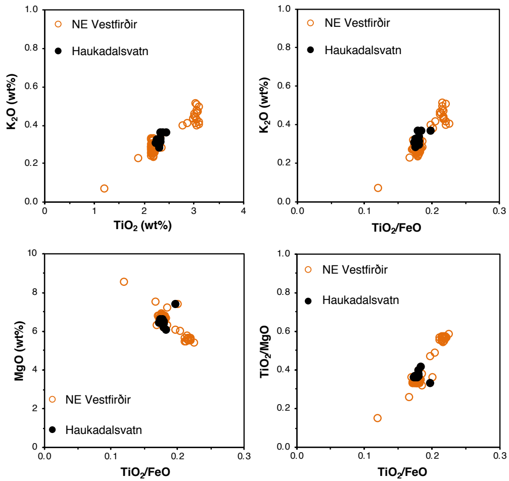
Figure S6.4: Bi-elemental plot comparisons demonstrating the correlation of the Grímsvötn BP-2 marker tephra in Haukadalsvatn (n=12) to the tephra layers found in Northwest Iceland lakes (n=68, Harning et al., 2018b).
