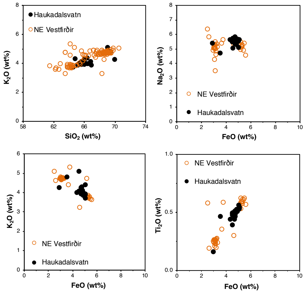
Figure S6.10: Bi-elemental plot comparisons demonstrating the correlation of the Snæfellsjökull-1 marker tephra in Haukadalsvatn (n=25) to the tephra layers found in Northwest Iceland lakes (n=33, Harning et al., 2018b).
