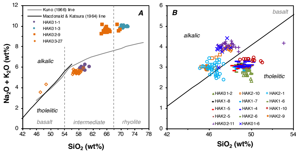
Figure 6.3: Marker tephra from Haukadalsvatn plotted on a total alkali vs silica (TAS) plot, where B) is a basalt confined TAS plot. The MacDonal and Katsura (1964) and Kuno (1966) lines separate alkalic from tholeiitic tephra.
