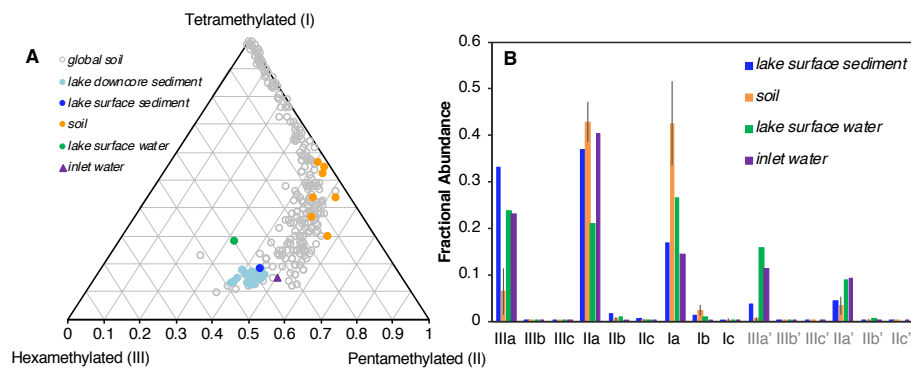
Figure 7.5: brGDGT fractional abundances for Skorarvatn lake sediment (n=31), soil (n=7), lake surface water (n=1) and inlet water (n=1). A) Total tetra-, penta-, and hexamethylated brGDGTs in comparison to the global soil dataset (n=239, De Jonge et al., 2014a), and B) All individual brGDGTs quantified. 6-methyl isomers denoted with prime symbol in gray.
