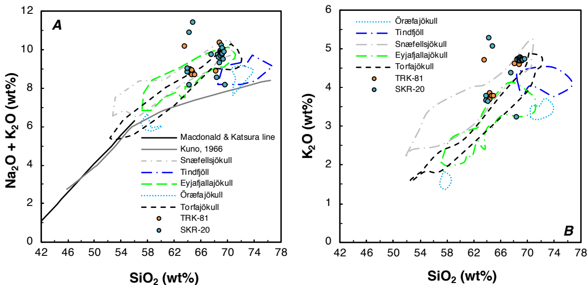
Figure 5.8: Examples of silicic tephra discrimination from Tröllkonuvatn and Skorarvatn. Both tephra are clearly alkalic and likely originated from Snæfellsjökull.
