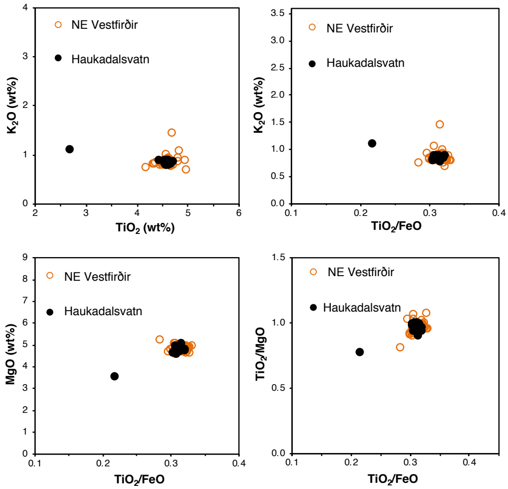
Figure S6.9: Bi-elemental plot comparisons demonstrating the correlation of the Katla 2190 marker tephra in Haukadalsvatn (n=28) to the tephra layers found in Northwest Iceland lakes (n=69, Harning et al., 2018b).
