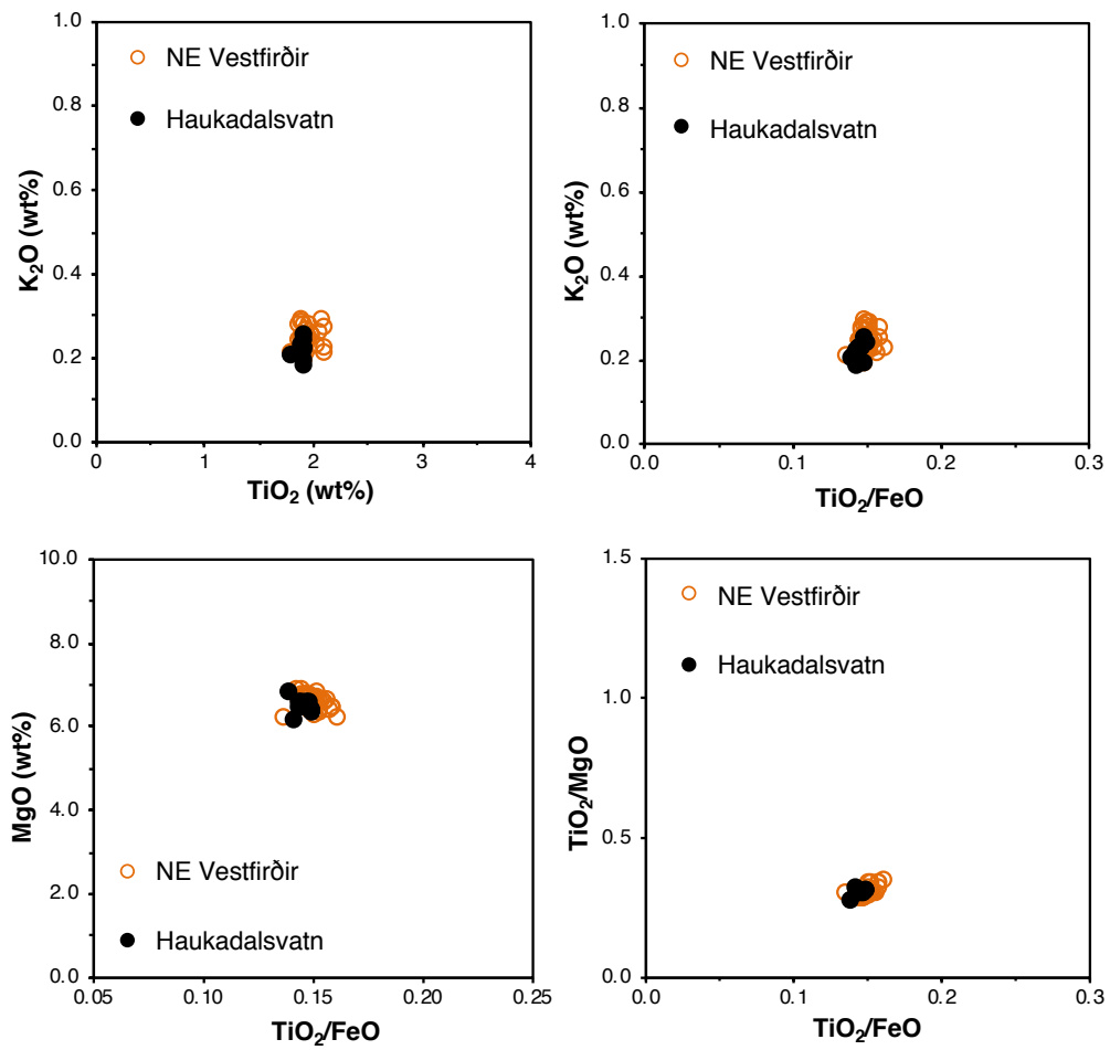
Figure S6.12: Bi-elemental plot comparisons demonstrating the correlation of the basaltic component Settlement Layer marker tephra in Haukadalsvatn (n=10) to the tephra layers found in Northwest Iceland lakes (n=44, Harning et al., 2018b).
