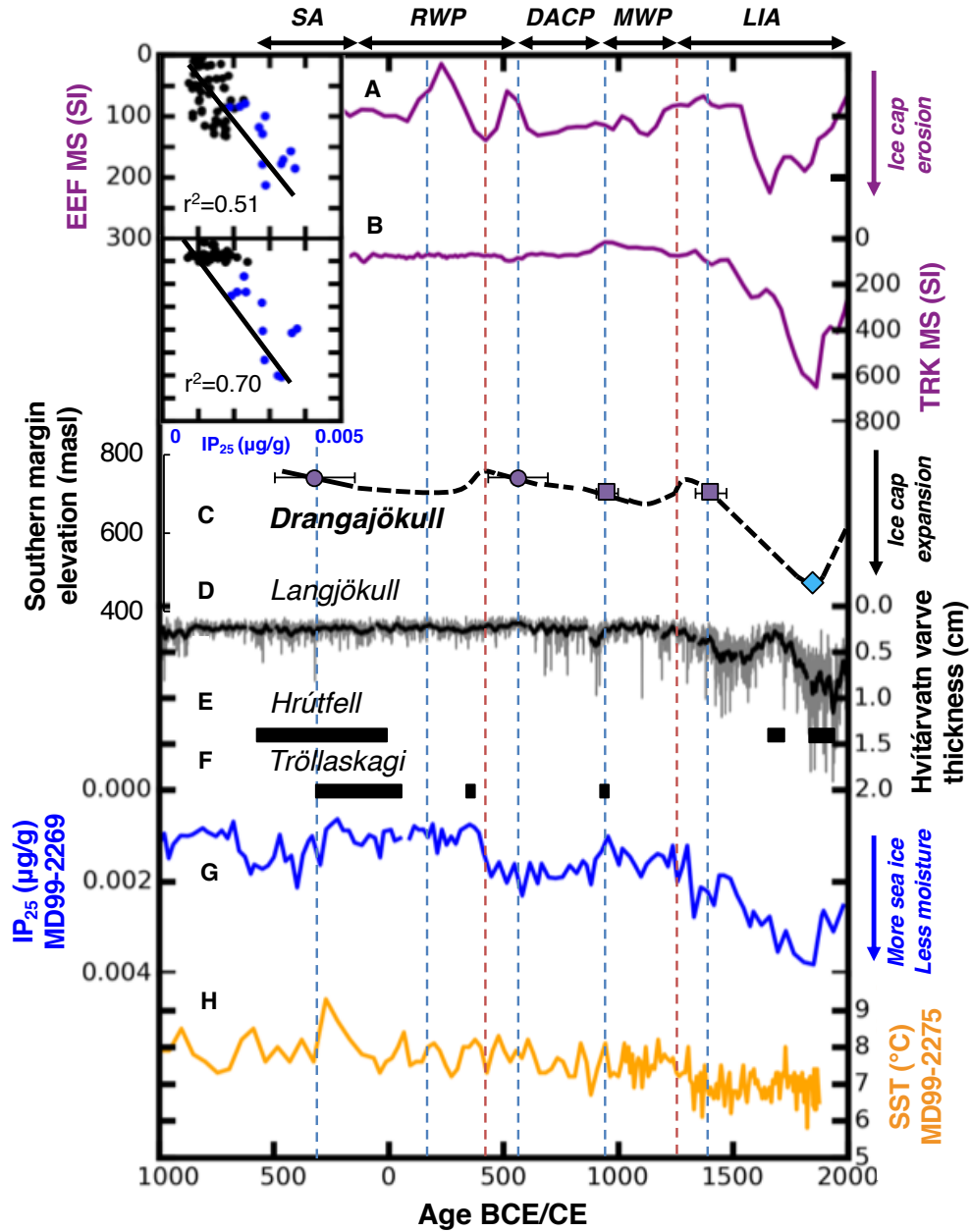
Figure 3.11: Glacial proxy records illustrated by inverted MS records from A) EEF and B) TRK, C) south margin elevation change, D) inverted Hvítárvatn varve thickness record (Larsen et al., 2011), E) Hrútfell moraine ages (Kirkbride and Dugmore, 2006), Tröllaskagi moraines (Stötter et al., 1999), G) inverted IP_{25} sea ice record from MD99-2269 on the North Icelandic Shelf (Cabedo-Sanz et al., 2016) and H) diatom-inferred SST record from MD99-2275 on the North Icelandic Shelf (Jiang et al., 2015). All records oriented down for cooler conditions. Blue (red) vertical lines represent episodes of Drangajökull advance (retreat). Insets (upper left): Biplots of MD99-2269 IP_{25} versus MS records from lakes EEF and TRK over the last 3 ka. All records were resampled to a common and uniform interval of 51 and 43 years, for EEF and TRK respectively, using the AnalySeries software package ( n = 69 , Paillard et al., 1996). Blue points highlight LIA conditions (1400 – 1850 CE) and black points for pre-LIA conditions (1000 BCE – 1400 CE).
