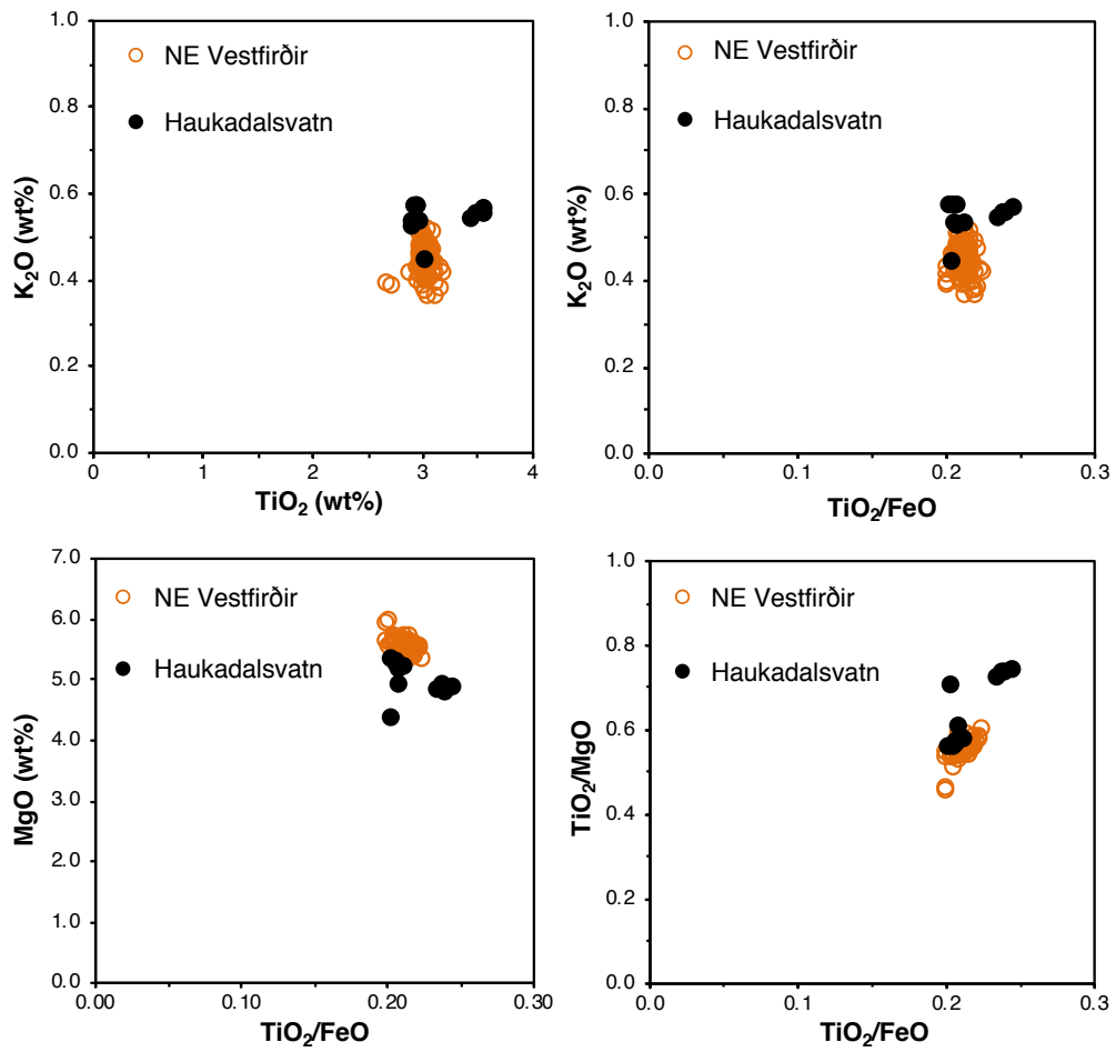
Figure S6.14: Bi-elemental plot comparisons demonstrating the correlation of the Grímsvötn B marker tephra in Haukadalsvatn (n=11) to the tephra layers found in Northwest Iceland lakes (n=94, Harning et al., 2018b).
