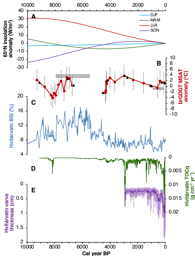
Figure 7.11: Comparisons of regional climate records to Fossrúfúlækur’s paleotemperature record. A) Seasonal insolation curves over the last 10000 years (Laskar et al., 2004), B) brGDGT MSAT anomaly
