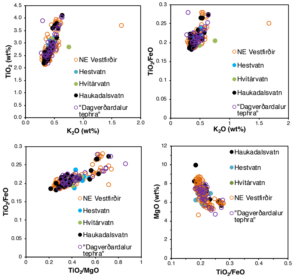
Figure S6.3: Bi-elemental plot comparisons demonstrating the correlation of the Hekla VF marker tephra in Haukadalsvatn (n=34) to the tephra layers found in Northwest Iceland lakes (n=113, Harning et al., 2018b), Hestvatn (n=12, Jóhannsdóttir, 2007), Hvítárvatn (n=6, Jóhannsdóttir, 2007) and the "Dagverðardalur tephra" (n= 34, Gudmundsdottir et al., 2018).
