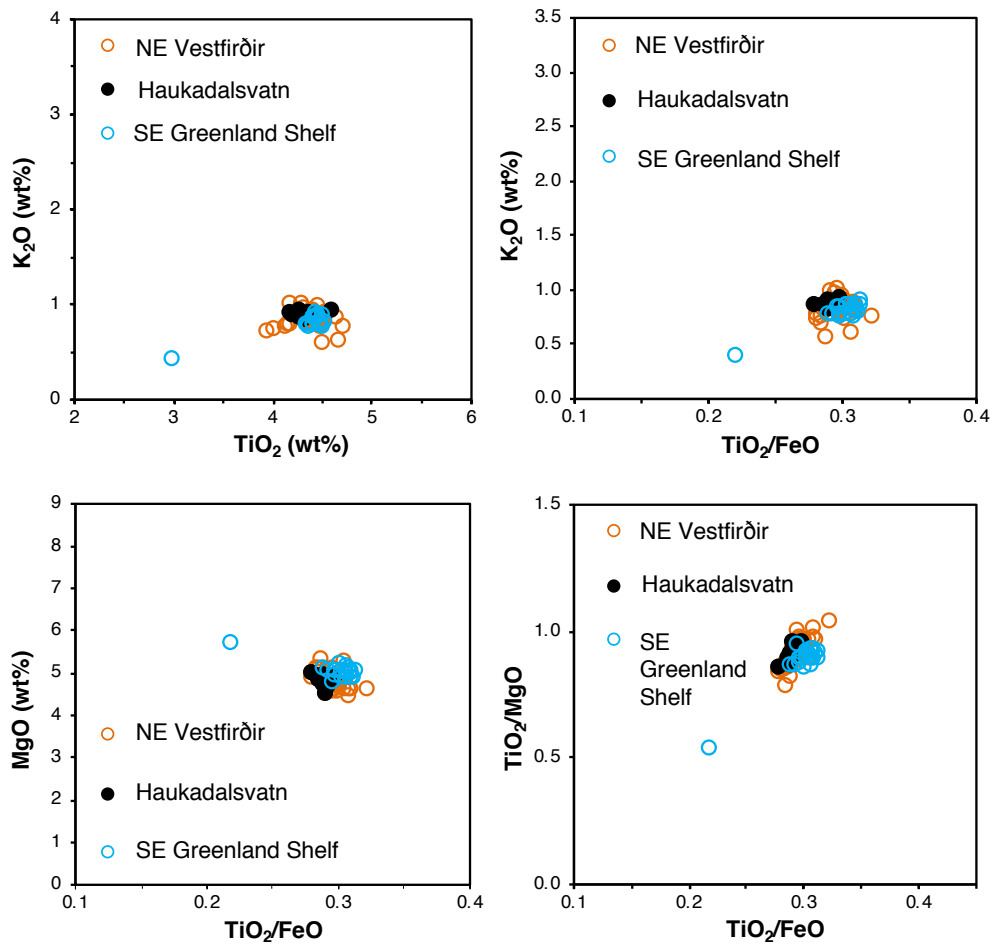
Figure S6.6: Bi-elemental plot comparisons demonstrating the correlation of the Katla EG marker tephra in Haukadalsvatn (n=12) to the tephra layers found in Northwest Iceland lakes (n=40, Harning et al., 2018b) and on the SE Greenland Shelf (n=20, Jennings et al., 2014).
