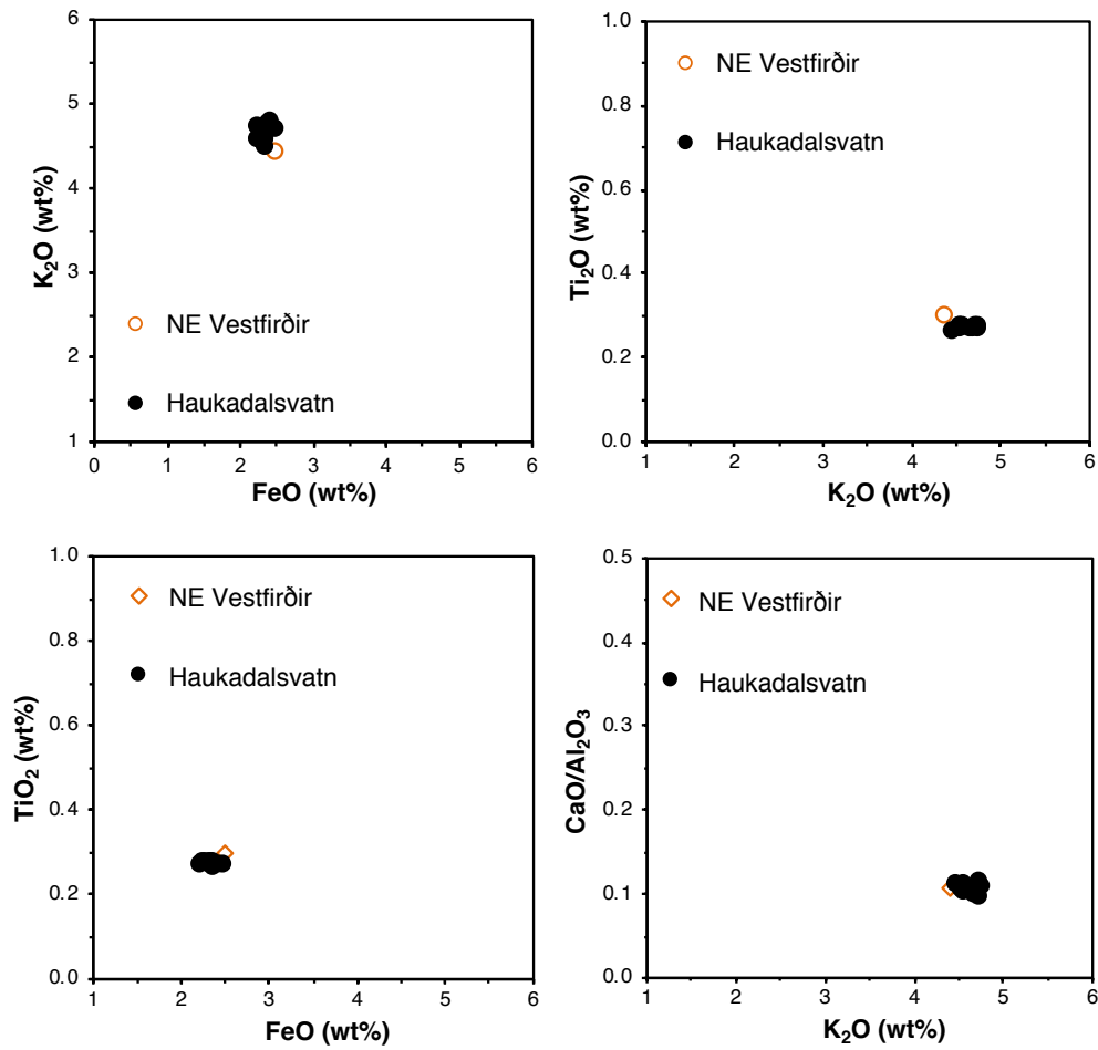
Figure S6.13: Bi-elemental plot comparisons demonstrating the correlation of the rhyolitic component Settlement Layer marker tephra in Haukadalsvatn (n=10) to the tephra layers found in Northwest Iceland lakes (n=1, Harning et al., 2018b).
