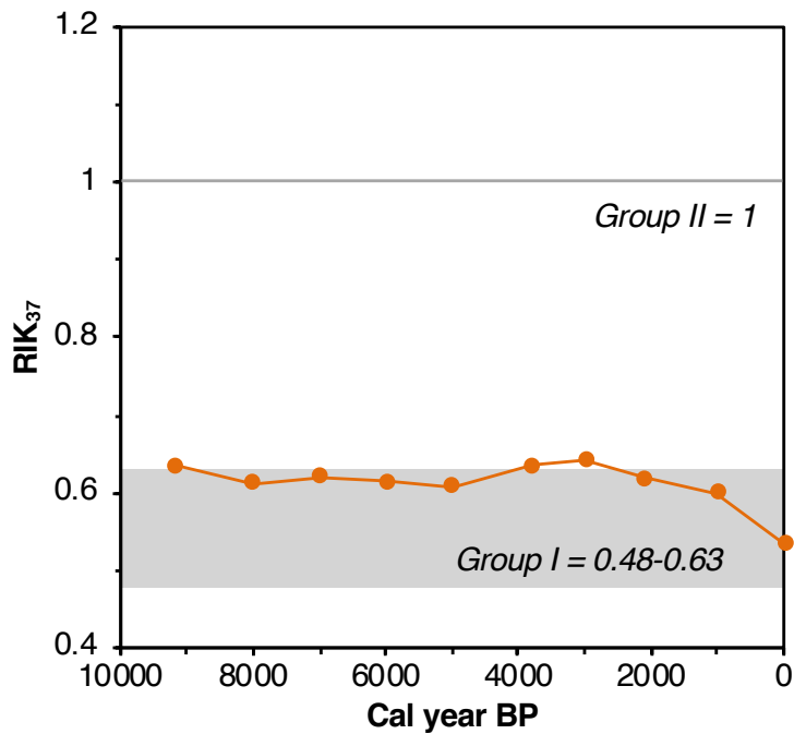
Figure 7.8: Alkenone haptophyte source based on RIK_{37} index (after Longo et al., 2018). RIK_{37} = (C_{37:3a}/C_{37:3a}+C_{37:3b}) , where values of 1 indicate Group II and values of 0.48- 0.63 indicate Group I haptophytes.
