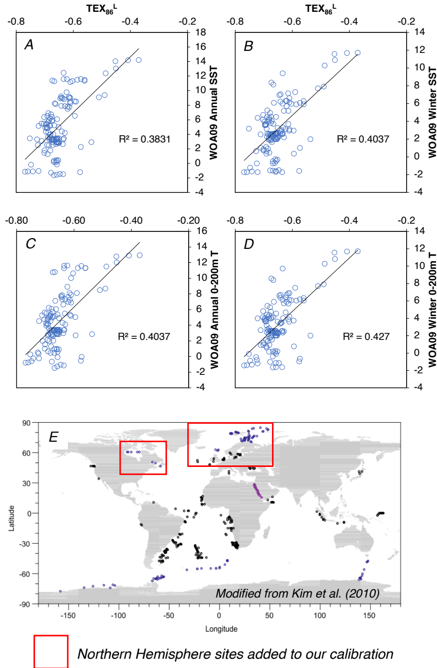
Figure S8.3: Using samples selected from the global calibration of Kim et al. (2010), we tested whether we could improve the local calibration by extending the range of samples, and thus, the environmental gradient. We applied the same calibration techniques as described for our local Icelandic calibration in the main text (Section 3.5). A) Annual SST, B) Winter SST, C) Annual 0-200 m T, and D) Winter 0-200 m T. The deviation from linearity and higher uncertainty of temperature estimates is clearly shown by the samples from the colder regions ( <5 °C) and concomitant lower TEX_{86}^L ratios. Panel E highlights the northern hemisphere samples included from the global calibration of Kim et al. (2010).
