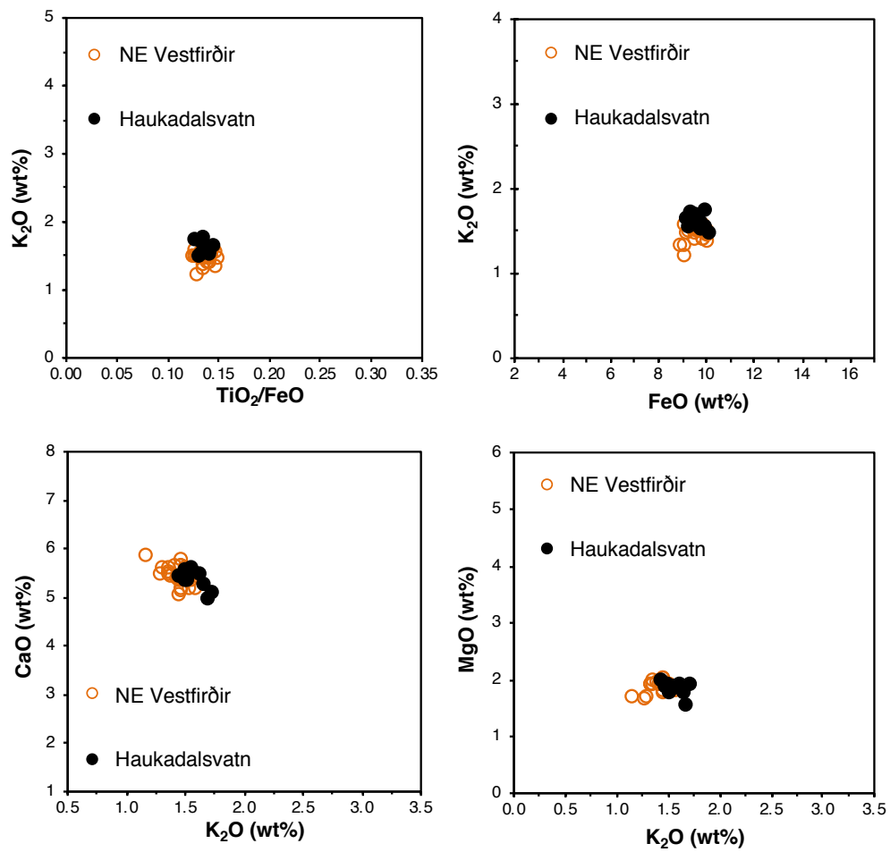
Figure S6.14: Bi-elemental plot comparisons demonstrating the correlation of the Hekla 1693 marker tephra in Haukadalsvatn (n=12) to the tephra layers found in Northwest Iceland lakes (n=29, Harning et al., 2018b).
