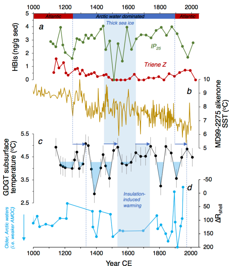
Figure 8.6: Comparison of select B997-316 GGC marine climate proxies to other well-dated, high-resolution Icelandic NIS marine climate records. A) B997-316 GGC IP_{25} and triene Z concentrations (this study), B) MD99-2275 alkenone-inferred SST (Sicre et al., 2011), C) B997-316 GGC GDCGT-inferred subsurface temperatures, with values below the record mean highlighted in blue (this study), and D) schlerochronological \Delta R record, where increases in \Delta R_{shell} values reflect the incursion of older, Arctic waters and a weaker AMOC (Wanamaker et al., 2012). Vertical blue bars highlight the period of interpreted thick sea ice, and then the delayed associated insulation/warming of the subsurface. Dashed blue lines bound the inferred periods of LIA-like conditions for the surface (A-B) and subsurface (C).
