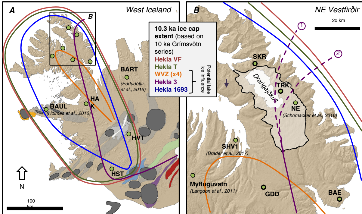
Figure 5.12: Estimated dispersal boundaries of select tephra. Limits based on the presence/absence of tephra in A) west Iceland lake sediment records and B) Vestfirðir lake sediment records and soils sites (green circles, Harðardóttir et al., 2001; Jóhannsdóttir, 2007; Langdon et al., 2011; Eddudóttir et al., 2016; Harning et al., 2016a, 2016b; Holmes et al., 2016; Schomacker et al., 2016; Brader et al., 2017; this study). HAK = Haukadalsvatn, HVT = Hvitárvatn, HST = Hestvatn. 10.3 ka extent of proto-Drangajökull delineation based on the presence/absence of the 10 ka Grímsvötn tephra series in a network of lake sediment and soil sites (Harning et al., 2016b).
