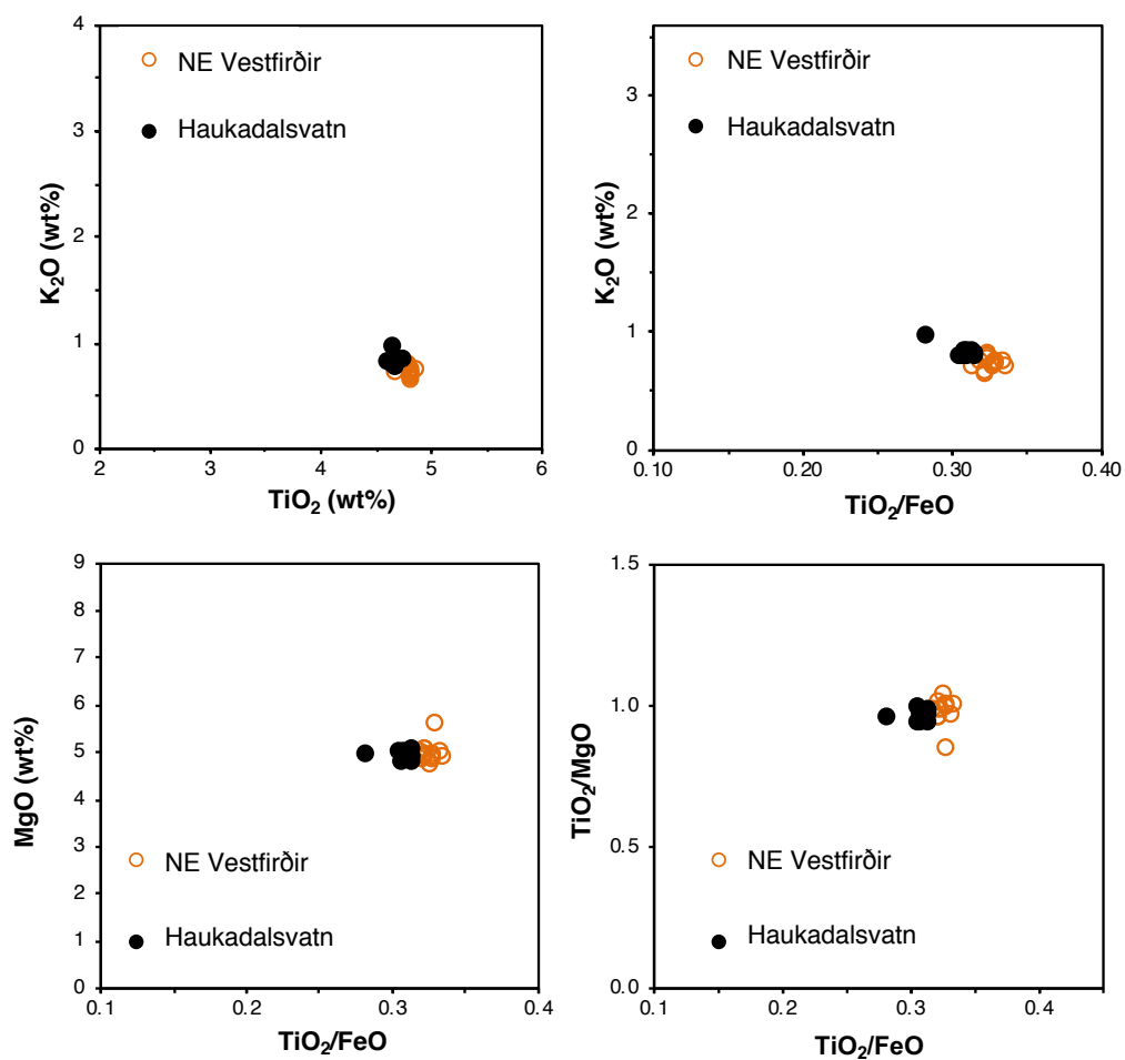
Figure S6.11: Bi-elemental plot comparisons demonstrating the correlation of the Katla 1260 marker tephra in Haukadalsvatn (n=10) to the tephra layers found in Northwest Iceland lakes (n=14, Harning et al., 2018b).
