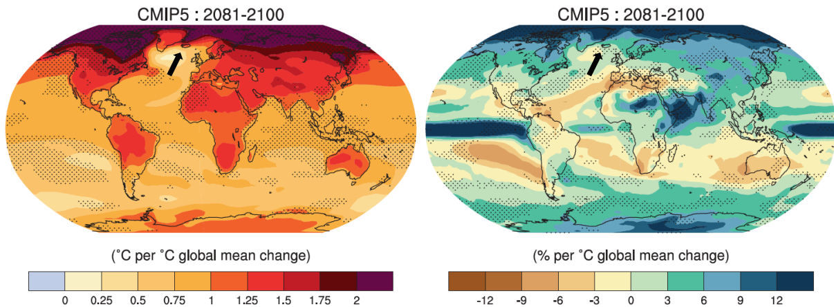
Figure 1.1: Projected °C (left) and percent (right) temperature increases relative to global mean change per the Coupled Model Intercomparison Project 5 (CMIP5). Iceland’s location along the periphery of strongest projected warming marked with a black arrow.
