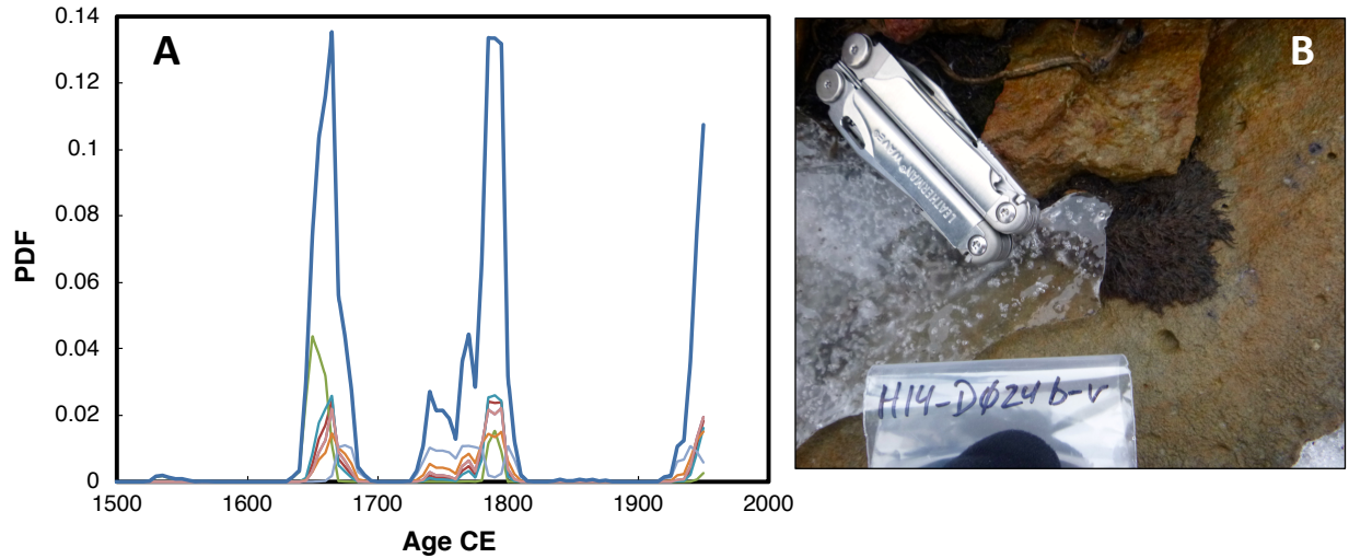
Figure 3.5: Individual probability distribution functions (PDF) of the 7 emerging dead vegetation samples with ^{14}\text{C} dates between 250 and 175 BP. Ages calibrated in OxCal 6.0 with the IntCal13 calibration curve (Bronk Ramsey, 2009; Reimer et al., 2013). A normalized sum of the individual PDFs is shown by the bold blue line. B) Example of dead vegetation sample (CURL-18810) emerging from the southern margin prior to sampling.
