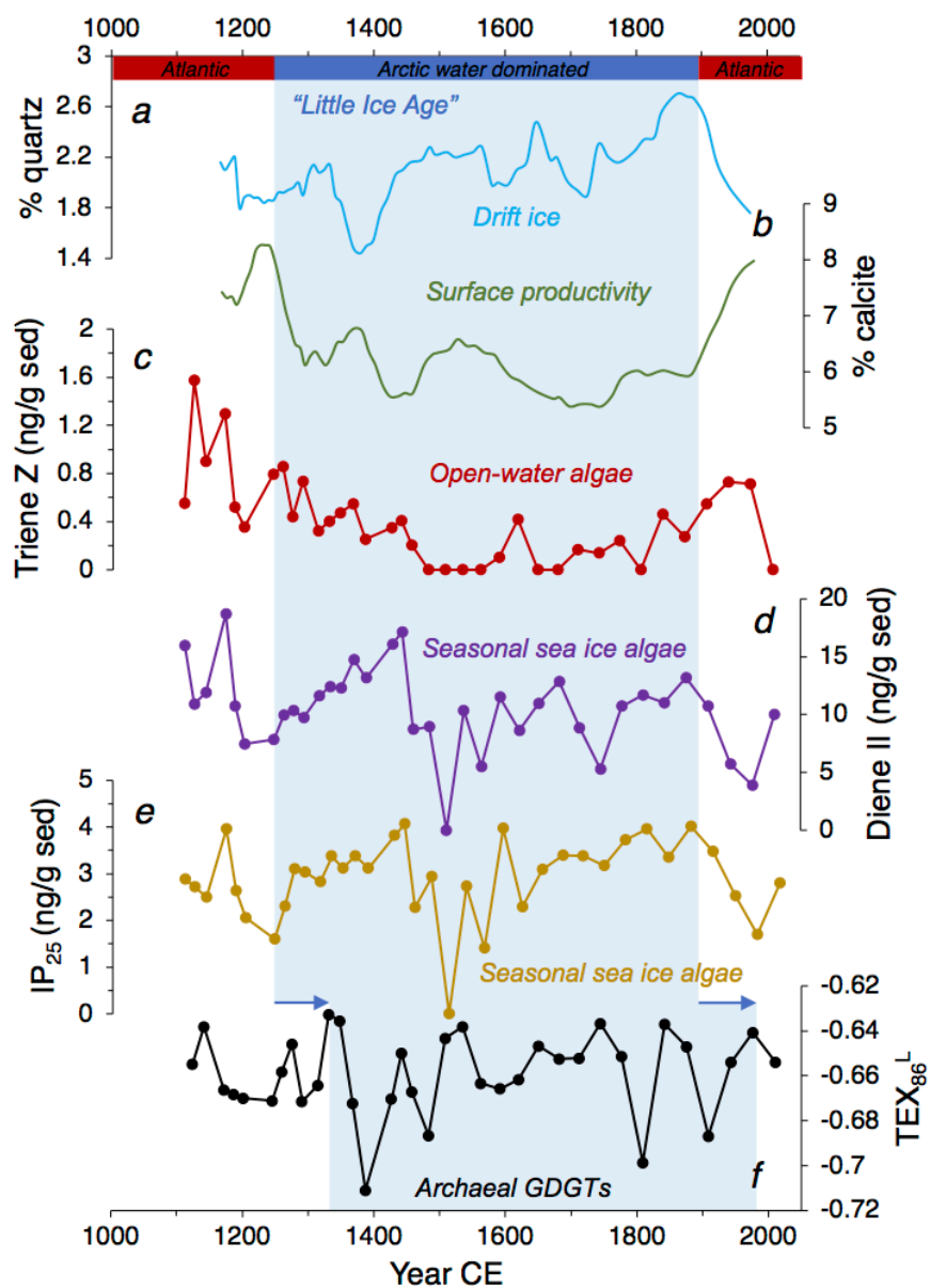
Figure 8.3: B997-316 GGC marine sediment core climate proxies over the last millennium. A) % quartz, B) % calcite, C) triene Z concentrations, D) diene II concentrations, E) IP 25 concentrations, and F) TEX 86 L . Blue boxes highlight colder, LIA-like conditions reflected in the surface climate proxies (A-E) and the subsurface proxy (F).
