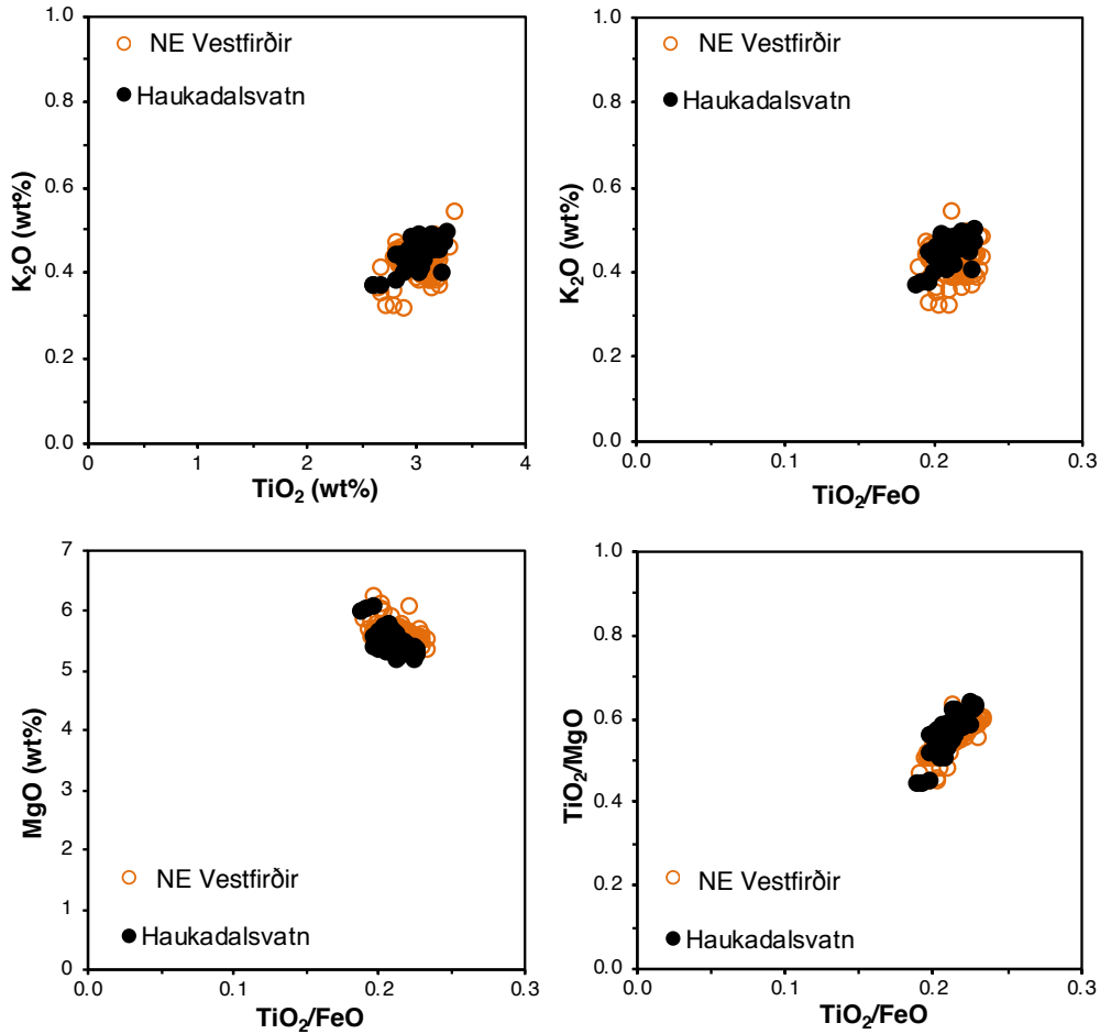
Figure S6.13: Bi-elemental plot comparisons demonstrating the correlation of the Grímsvötn 10 ka Series marker tephra in Haukadalsvatn (n=81) to the tephra layers found in Northwest Iceland lakes (n=122, Harning et al., 2018b).
