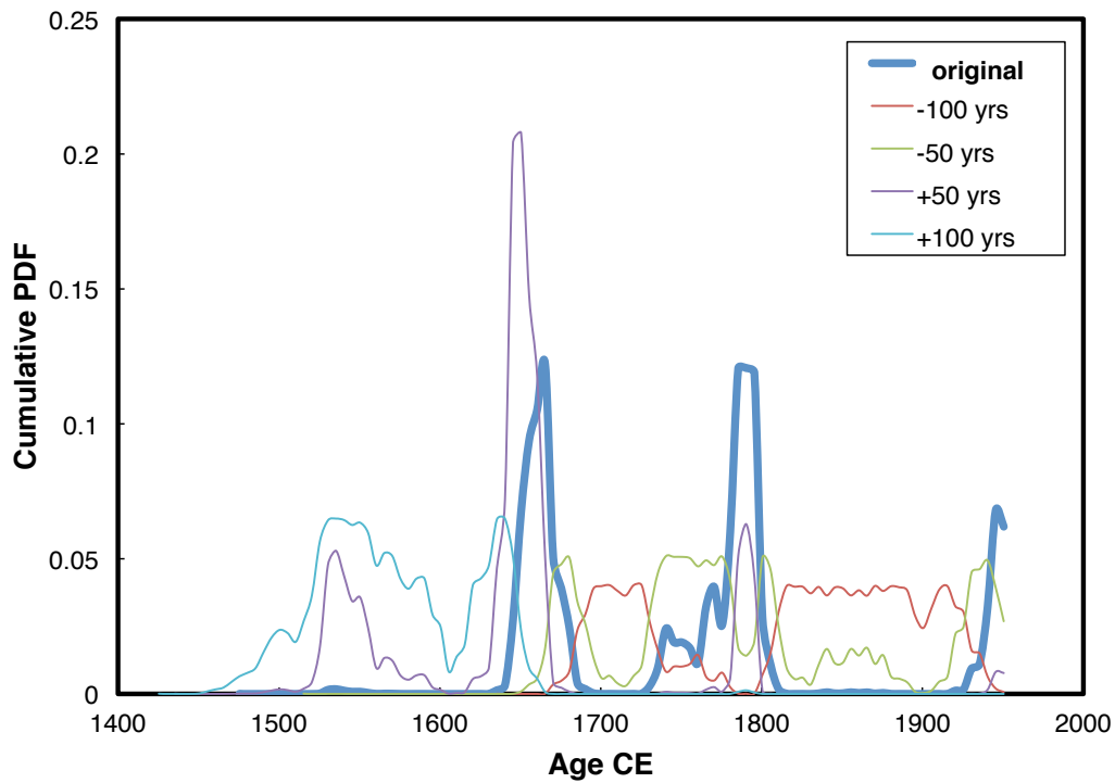
Figure S3.1: Plot of the original calibrated cumulative PDF (bold blue line) for the 7 emerging dead vegetation samples with ^{14}\text{C} dates between 250 and 175 BP. By altering the original ^{14}\text{C} dates by -100, -50, +50 and +100 years and summing the new individual PDFs from recalibrated ages, we show that the three peaks revealed in the original cumulative PDF are unique and not an artifact of the Late Holocene's variable calibration curve.
