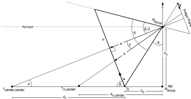
Fig. 10. FOV and accompanying variables used to calculate d and \psi .
