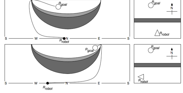
Fig. 9. Translational oscillation induced in the Cylindrical planner by a long thin wall. The initial path around the wall (top), and the path at a later time (bottom).
