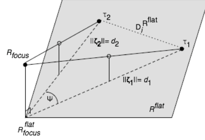
Fig. 2. Calculation of D_i^{R^{flat}} . R_{focus} is the focal point of the robot's camera array. \tau_1 and \tau_2 are the endpoints of i projected onto R^{flat} .
