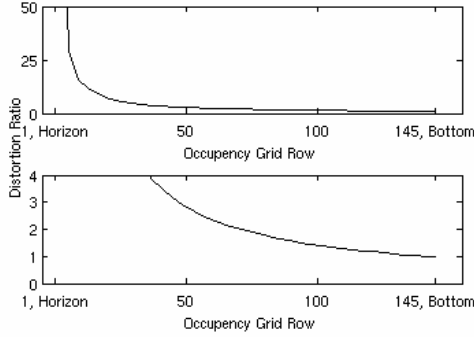
Fig. 8. Distortion ratio ( D_i^{R^{flat}} for vertical neighbors divided by D_i^{R^{flat}} for the bottom two vertical neighbors. Note that this is proportional to D_i^{R^{flat}}/D_i^O .) as a function of occupancy grid row (top). Close up of distortion ratio (bottom).
