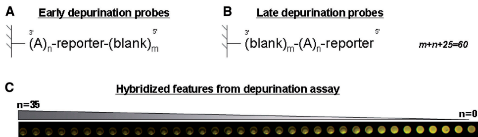
Figure 2. Hybridization based depurination assay. A hybridization based depurination assay was used to measure the extent of the depurination side reaction during synthesis of microarrays using the legacy process. The depurination probes are composed of a depurination sensitive stilt of variable length ( A_n , n = 10-35 ) and a common 25mer reporter sequence. The length of each depurination probe is n + 25 and their synthesis was staggered during the 60-nt synthesis cycles used to synthesize the 60mer microarray. Early depurination probes ( A ) are such that their synthesis is initiated as early as possible, i.e. m blank synthesis cycles are performed after the probe synthesis so that m + n + 25 = 60 . Late depurination probes ( B ) are such that their synthesis is initiated as late as possible, i.e. m blank synthesis cycles are performed prior to the probe synthesis so that m + n + 25 = 60 . All probes are synthesized simultaneously and hybridized to a labeled oligonucleotide complementary to the reported probe. The early depurination probe hybridization signals show a decrease in signal intensity with increasing number of n due to a loss of reporter probe ( C ). A similar profile is observed for late depurination probes.
