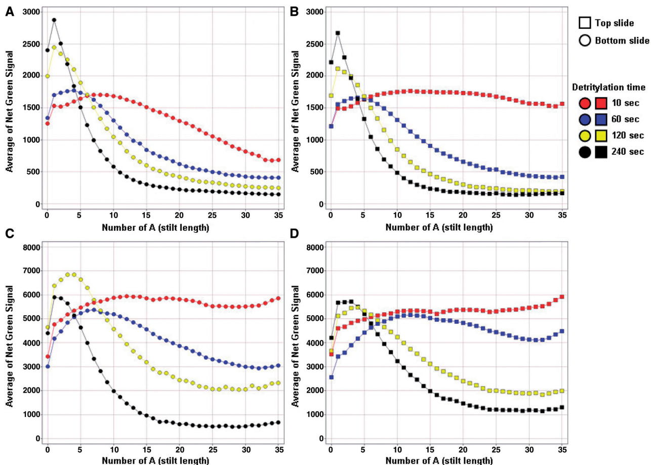
Figure 3. Signal profiles of depurination probes and the effect of slide location on the wafer and detritylation time. Representative signal profiles of the depurination probes manufactured with the legacy process are plotted as a function of the number n of A nucleobases in the depurination stilt for early ( A and B ) and late ( C and D ) depurination probes were described in Figure 2A and B). The shape of the depurination intensity profiles are characterized by a decrease in signal after the signal reaches a maximum. This loss in signal is consistent with the loss of the reported probe following depurination-induced cleavage in the A nucleobase stilt. The signal decrease is correlated with the detritylation time, with higher detritylation times resulting in steeper declines past the maximum signal. Additionally, the profiles for slides synthesized close to the bottom port, also called bottom slide ( A and C ) have significantly higher signal loss than the profiles of slides synthesized close to the top port, also called top slide ( B and D ).
