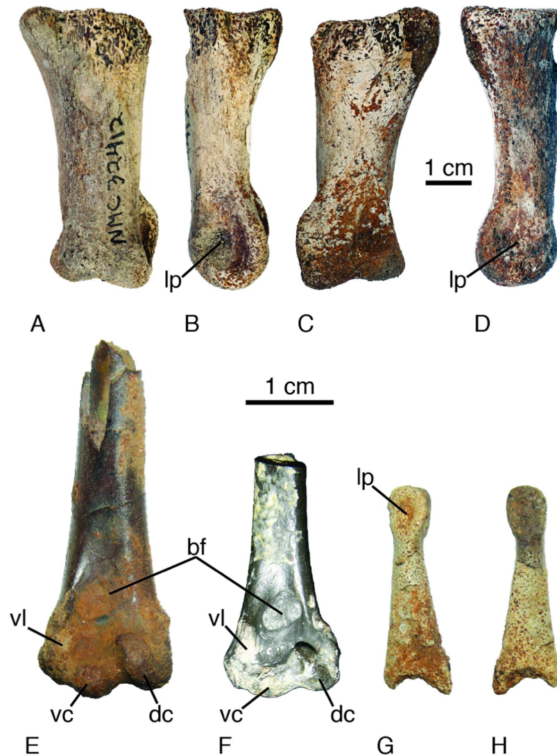
Figure 2. The Ellesmere Island avian fossils. The (probable) left proximal phalanx of digit IV from Gastornis sp. (CMNFV 32412): (A) dorsal view, (B) lateral view, (C) plantar view, and (D) medial view. The distal humeri of Presbyornis : (E) CMNFV 53369 from the Margaret Formation of Ellesmere Island, Canada, and (F) University of California Museum of Paleontology UCMP 119395 from the Wasatch Formation of Wyoming, USA in cranial view. The (G) right and (H) left surfaces of the indeterminate avian pedal phalanx (CMNFV 53368) showing the extensive sand pitting on the surface. Abbreviations: bf, brachial fossa; dc, dorsal condyle; lp, collateral ligament pit; vc, ventral condyle; and vl, facet for the ventral collateral ligament on the ventral supracondylar tubercle.
