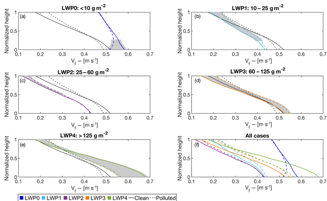
Figure 3. Vertical profiles of 120 min time-averaged mean Doppler velocity for clean and polluted conditions for (a) LWP0, (b) LWP1, (c) LWP2, (d) LWP3, (e) LWP4 and (f) all LWP bins. The black reference lines in each panel represent the mean profiles for all the LWP bins. Grey shading represents regions of the cloud layer where there is a statistically significant difference between the clean and polluted V_f distributions.
