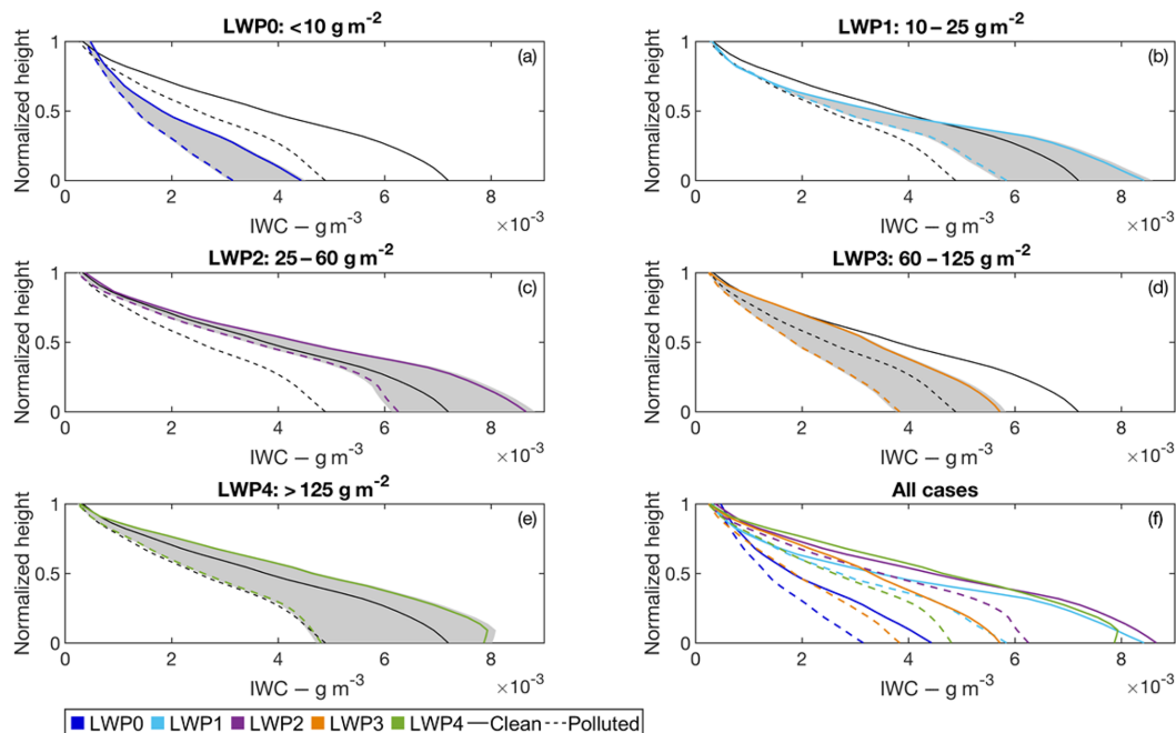
Figure 2. Vertical profiles of ice water content for clean and polluted conditions, as in Fig. 1, for (a) LWP0, (b) LWP1, (c) LWP2, (d) LWP3, (e) LWP4 and (f) all LWP bins. The black reference lines represent the mean profiles for all the LWP bins. Grey shading represents regions of the cloud layer where there is a statistically significant difference between the clean and polluted IWC distributions.
