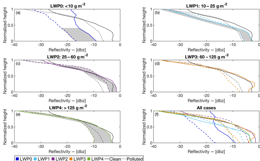
Figure 1. Reflectivity profiles for the five LWP regimes for (a) LWP0, (b) LWP1, (c) LWP2, (d) LWP3, (e) LWP4 and (f) all LWP bins. Zero (0) corresponds to cloud base, and 1 corresponds to cloud top. Dashed lines represent polluted clouds, and solid lines indicate clean cases. The black lines, shown for reference in each panel, represent the mean profiles for the combined LWP bins. Grey shading represents regions of the cloud layer where there is a statistically significant difference between the clean and polluted reflectivity distributions.
