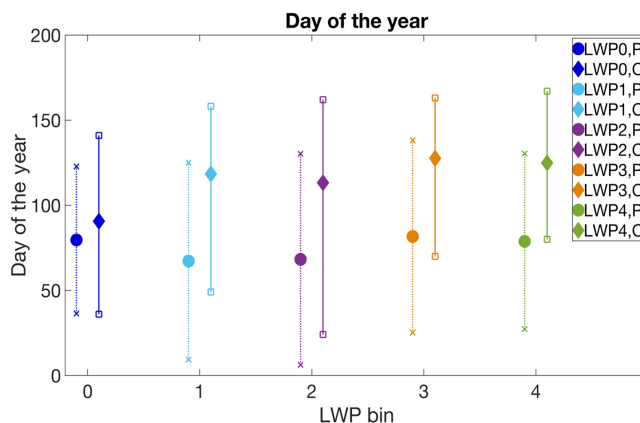
Figure 7. Mean day of sample for the distribution of sampled profile for clean and polluted clouds for each LWP scenario. Diamond markers with solid line indicate clean clouds; circle markers with dashed line represent polluted cases. The bars span the 20–80th percentile of the day-of-year distribution for each bin.
