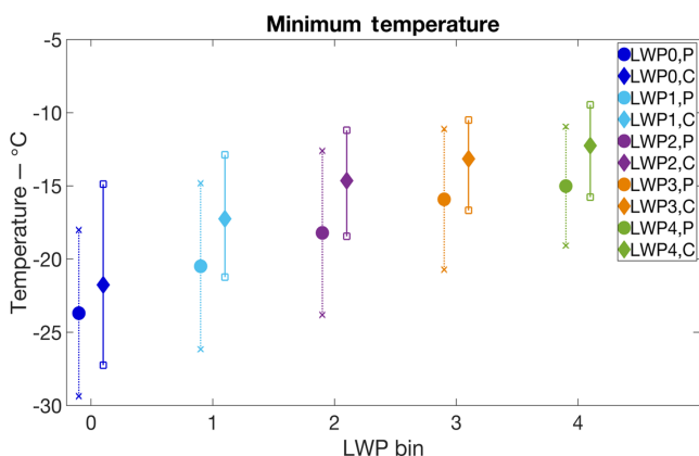
Figure 5. Mean minimum cloud temperature for clean and polluted clouds for each LWP bin. Diamond markers with solid line indicate clean clouds; circle markers with dashed line represent polluted cases. The bars span the 20–80th percentile of the T_{\min} distribution for each bin.
