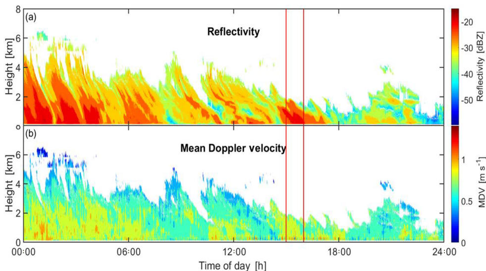
Figure 4. (a) Reflectivity and (b) mean Doppler velocity from the MMCR for a LWP0 cloud on 19 January 2006. Time from hours 15 to 16, marked between the red vertical lines, is the sample period used in this analysis.
