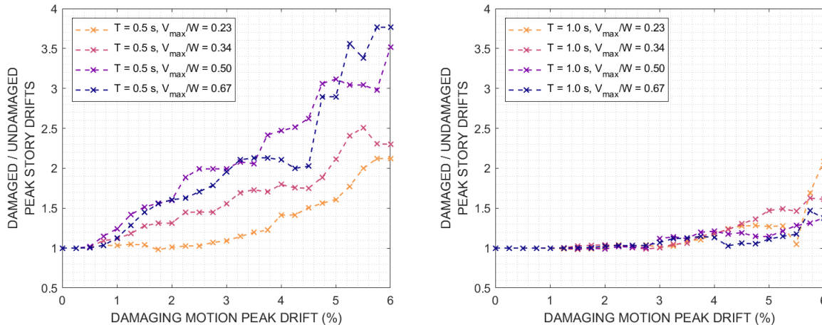
Figure 2.11: Median drift amplifications for SDOF models with variation strength and a first mode period (a) T = 0.5 s, and (b) T = 1.0 s.
