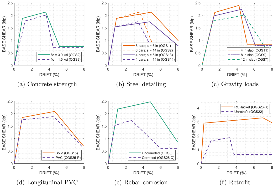
Figure 3.15: Static pushover response of columns configurations.
