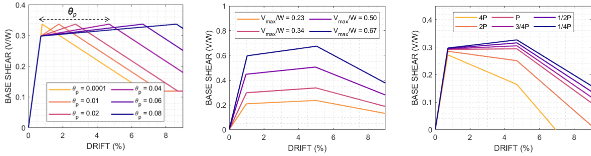
Figure 2.6: Static pushover response of SDOF models with (a) varied deformation capacity ( \theta_p ) and constant strength and stiffness, and (b) varied strength and stiffness with constant yield and capping drifts, and (c) P - \Delta effects.
