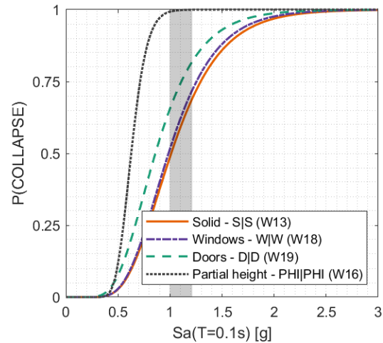
Figure 3.26: Collapse fragilities for walls with openings
