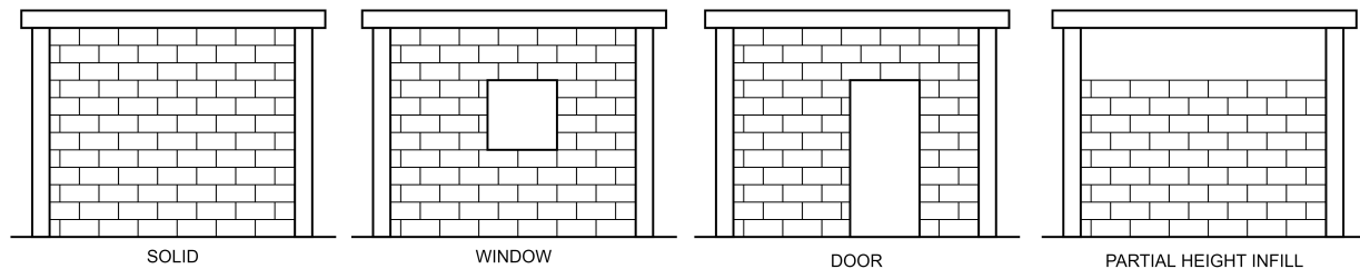
Figure 3.8: Masonry wall configurations with and without openings
