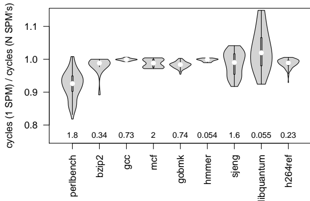
Figure 5. The effect on a benchmark’s performance (total cycles) as we collect additional software metrics.
