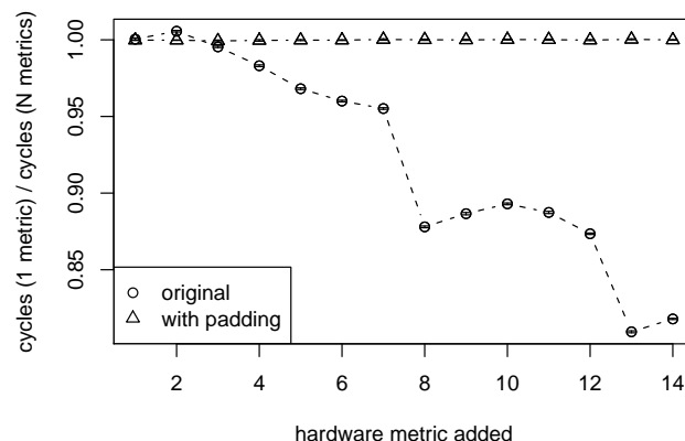
Figure 12. Change in h264ref’s total cycles as we add hardware metrics.
