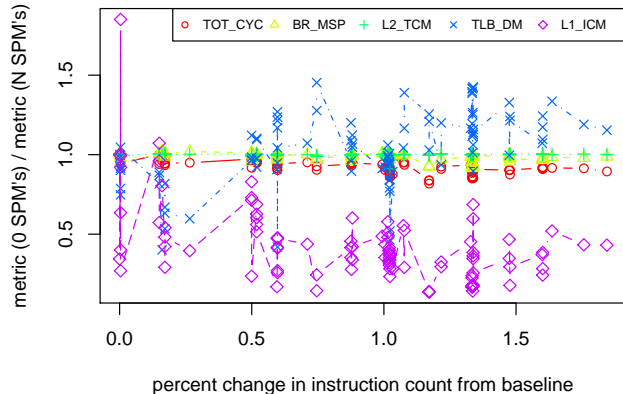
Figure 4. The effect on a hardware metric’s value for perlbench as we collect additional software metrics.
