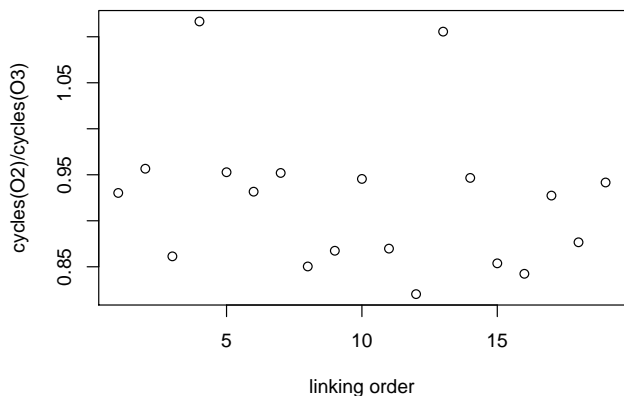
Figure 11. The effect of linking order on speedup of O3 over O2 for the bzip2 benchmark on m5 simulator.
