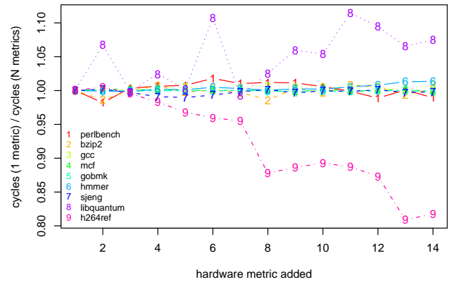
Figure 2. The effect on a benchmark’s performance (total cycles) as we collect additional hardware metrics.
