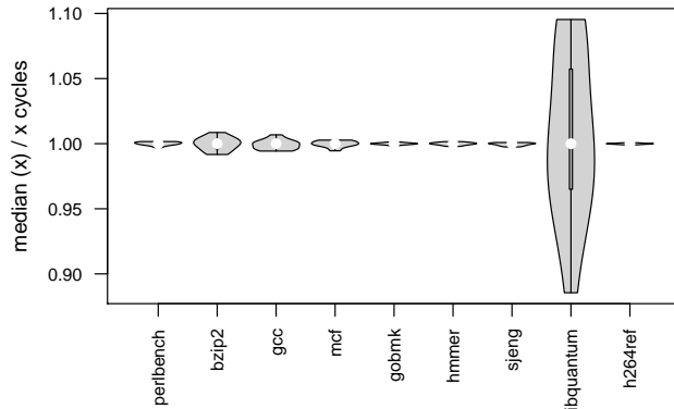
Figure 1. Variation of execution time (in cycles) across runs of the SPECint C 2006 benchmarks.
