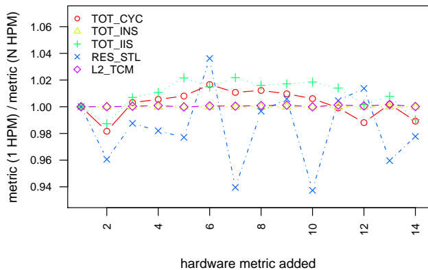
Figure 3. The effect on a hardware metric’s value for perlbench as we collect additional hardware metrics.
