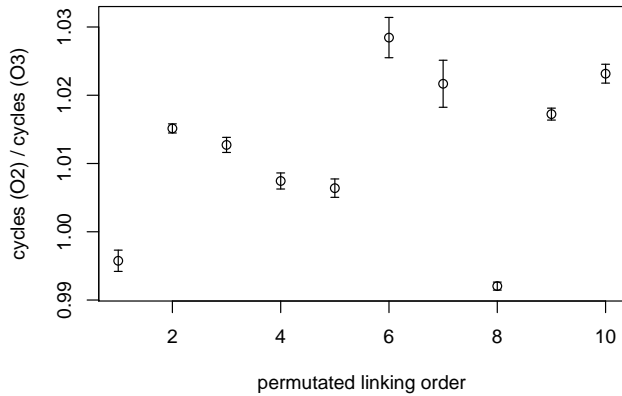
Figure 8. The effect of linking order on speedup of O3 over O2 for the perlbench benchmark.
