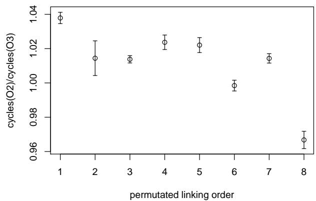
Figure 10. The effect of linking order on speedup of O3 over O2 for the perlbench benchmark on Core Duo workstation.
