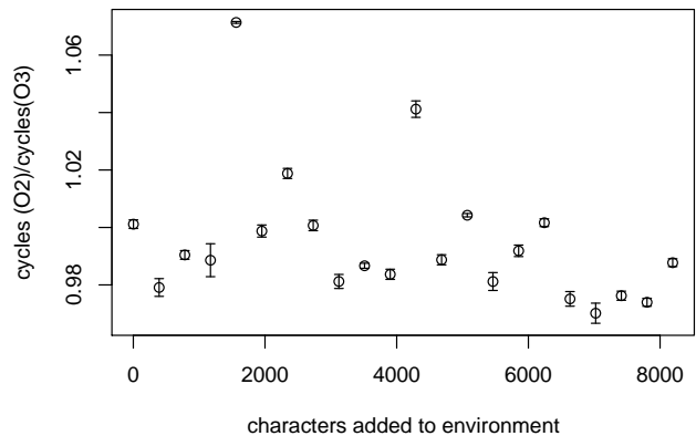
Figure 6. The effect of adding environment variables on the speedup of O3 over O2 for Perlbench.
