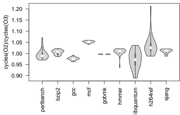
Figure 7. The effect of adding environment variables on speedup of O3 over O2 for our benchmarks.
