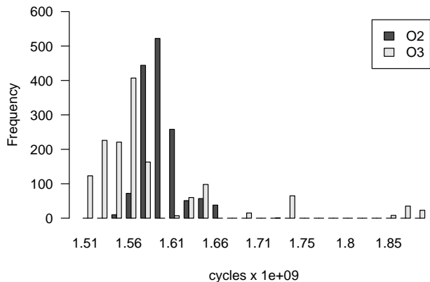
Figure 13. Using variant generation to determine the speedup of O3 over O2 . At a 95% confidence interval, we estimate the speedup to be 1.007 \pm 0.003
