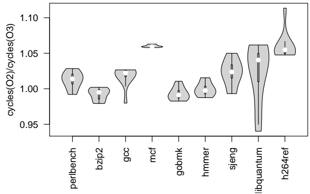
Figure 9. The effect of linking order on speedup of O3 over O2 for the SPECint benchmarks.
