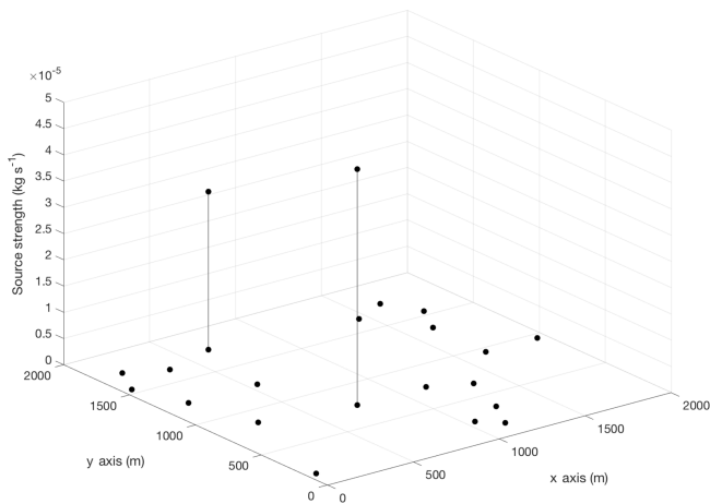
Figure 1. Synthetic test observation area: 2 km \times 2 km domain with 20 source locations (black dots) at randomly distributed x and y locations (position shown on x and y axes). Of 20 point sources, well site 6 ( x = 750 , y = 750 ) and well site 19 ( x = 650 , y = 1750 ) have non-zero source strengths (shown on the z axis).
