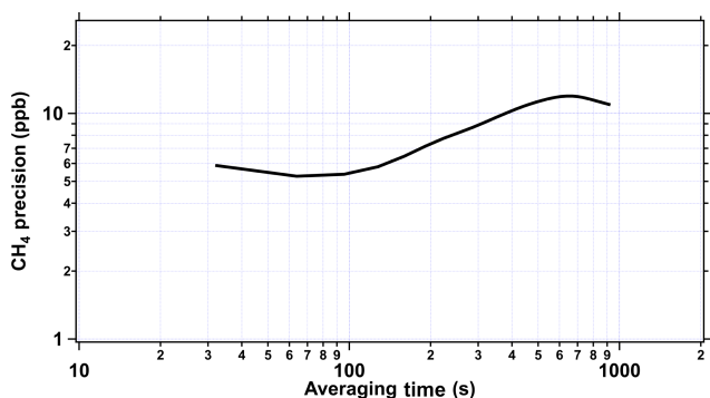
Figure 9. Allan deviation plot showing changes in measurement precision with averaging time from field data collected at Table Mountain on 26 January 2017.
