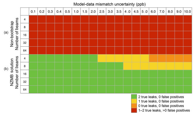
Figure 4. Summary of synthetic data test results. Top 5 rows show results of non-bootstrap inversions and bottom 5 rows show results of NZMB inversions for the 4, 8, 16, 32, and 64 beam cases. Columns indicate results for different values of model–data mismatch added as noise to the synthetic measurements. Color coding of cells indicates summary of model success, as detailed by the legend.
