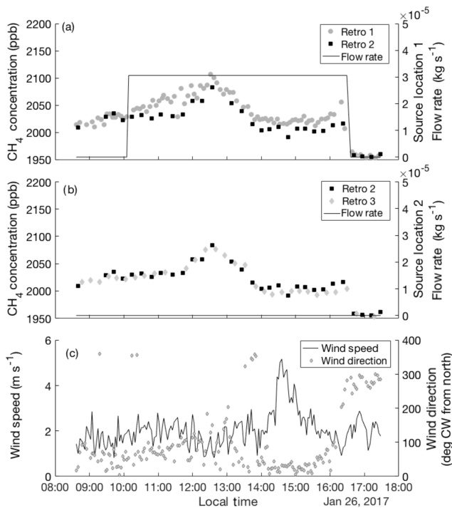
Figure 10. Line-integrated atmospheric \text{CH}_4 concentrations measured on 26 January 2017 along beam paths to retroreflectors 1 and 2 (a) and to retroreflectors 2 and 3 (b), as well as wind speed and wind direction (c). Gray and black points and left-hand axes of panels (a) and (b) show \text{CH}_4 concentration. The black line and right-hand axis in panel (a) show the flow rate at source location 1 (bounded by retroreflectors 1 and 2) and the black line and right-hand axis in panel (b) show the flow rate at source location 2 (bounded by retroreflectors 2 and 3). In panel (c), the black line and left-hand axis show wind speed and the gray diamonds and right-hand axis show wind direction (according to meteorological convention, 0^\circ is north, 90^\circ is east, 180^\circ is south, 270^\circ is west, and 360^\circ is north). All data reflects 2 min averaging time.
