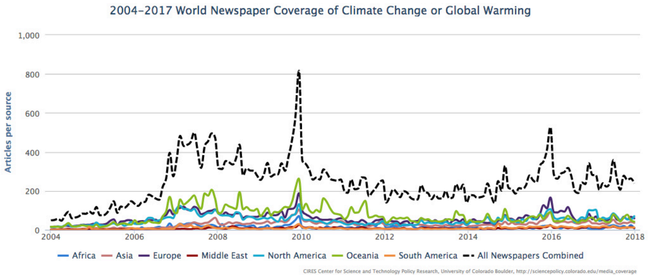
Figure 1: Media coverage of climate change or global warming in fifty-two sources across twenty-eight countries in seven different regions around the world, from January 2004 through December 2017.
