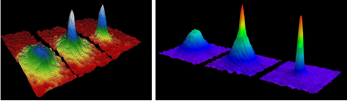
Figure 2.3: Images from the first BEC experiments of ^{87}\text{Rb} at JILA (left) and ^{23}\text{Na} at MIT (right). From left to right in each image, surface plots are shown of velocity distributions and real-space distributions, respectively, at temperatures just above, at, and below the critical temperature for BEC. The sharpening of the distribution below the critical temperature provides evidence BEC formation. Figures used with permission of E. A. Cornell from [67] (left) and W. Ketterle from [68] (right).
