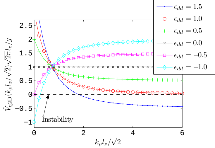
Figure 4.1: The quasi-2D momentum-space interaction potential (4.24) for fixed contact interaction coupling and various valued of the dipole interaction strength \epsilon_{dd} . The black dashed line marks \tilde{V}_{\text{q2D}}(k_\rho l_z / \sqrt{2}) = 0 , below which instabilities are possible. For \epsilon_{dd} = 0 , corresponding to no dipole interactions, the interaction is independent of momentum.
