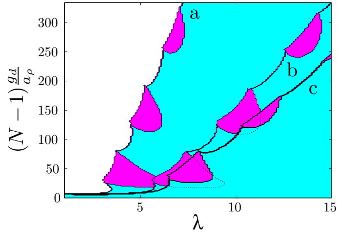
Figure 8.3: Structure/stability diagram for a single dipolar BEC. The colored regions indicate a dynamically stable condensate, and the pink (darker) regions indicate parameters for which the dipolar BEC has biconcave density. (a) and (b) are calculated using the ansatz for the axial wave function given in Eq. (8.7) and (c) is calculated using a full numeric grid. For (a), A_2 = 0 and l_z/a_z = 1 , and for (b), A_2 and l_z are treated variationally.
