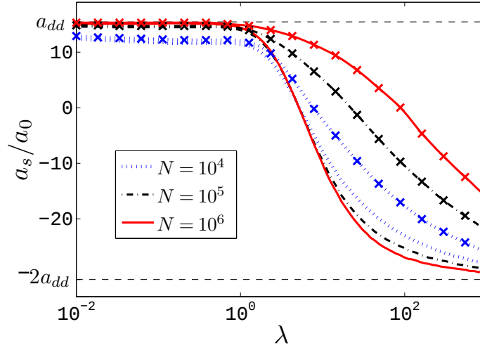
Figure 6.3: For a dipolar BEC of atomic ^{52}\text{Cr} , this figure illustrates the critical s -wave scattering length (below which the dipolar BEC is unstable) as a function of trap aspect ratio \lambda in units of the Bohr radius for \bar{\omega} = 2\pi \times 700 \text{ Hz} . The blue (dotted), black (dot-dashed) and red (solid) lines correspond to N = 10^4 , N = 10^5 and N = 10^6 , respectively. The lines without crossed symbols are the results of the Gaussian ansatz and lines with crossed symbols are the results of the exact solution of the GPE. Notice how, as N is increased, the Gaussian ansatz predicts a more stable condensate while the exact solution predicts a less stable condensate.
