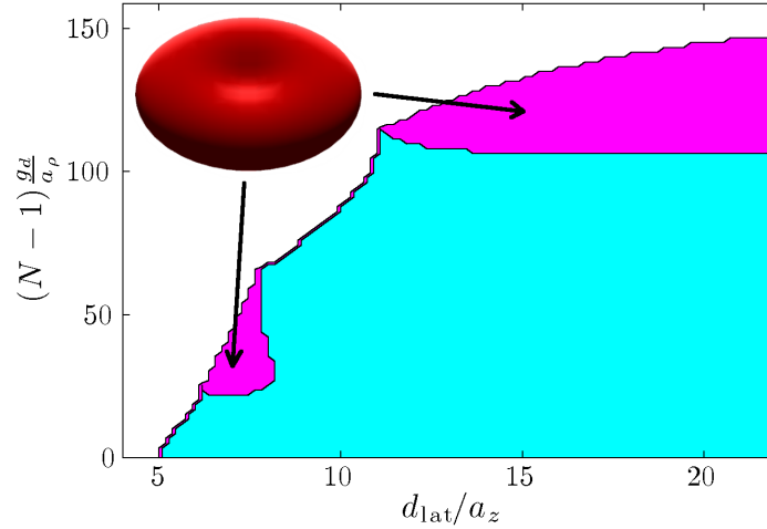
Figure 8.4: Structure/stability diagram for an infinite lattice of dipolar BECs in traps with aspect ratio \lambda = 10 as a function of lattice spacing d_{\text{lat}}/a_z and interaction strength (N-1)g_d/a_\rho . The colored region indicates dynamic stability, while the pink (darker) regions indicate parameters where the dipolar BECs have biconcave density. The inset shows an isodensity plot of a dipolar BEC with biconcave density.
