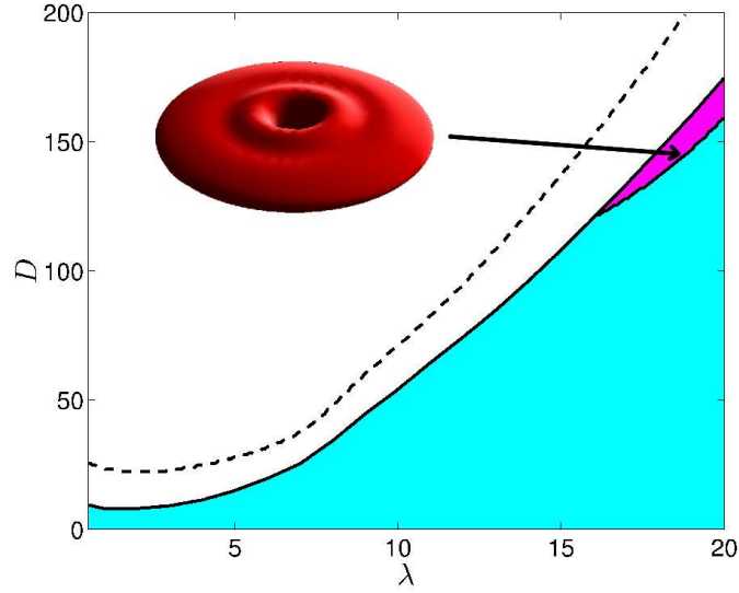
Figure 5.5: The black dashed line marks the maximum dipole strength D , for a given trap aspect ratio \lambda , above which the cylindrically symmetric Gross-Pitaevskii energy functional has no minimum corresponding to the s = 1 dipolar BEC. The solid line marks a more restrictive stability line, determined by the onset of dynamical instability, signaled by the emergence of an imaginary energy in an excitation mode. The pink (darker) region represents where radial oscillations with local minima are observed on dynamically stable states. The inset is an isodensity surface plot of an s = 1 dipolar BEC at the point in parameter space indicated by the arrow. The ripples in the density are explained in section 5.5.
