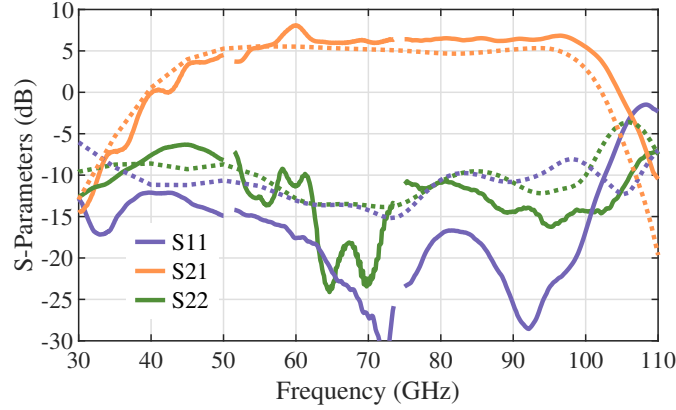
Figure 2.22: Measured (solid) and simulated (dashed) S-parameters of the cascode MMIC amplifier from Fig. 2.21. Circuit is biased with V_D = 12V , I_D = 38mA .
