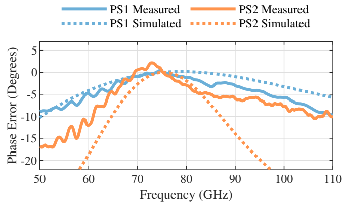
Figure 4.12: Simulated and measured phase error of the 90° and the 180° reflective phase shifters shown over frequency.
