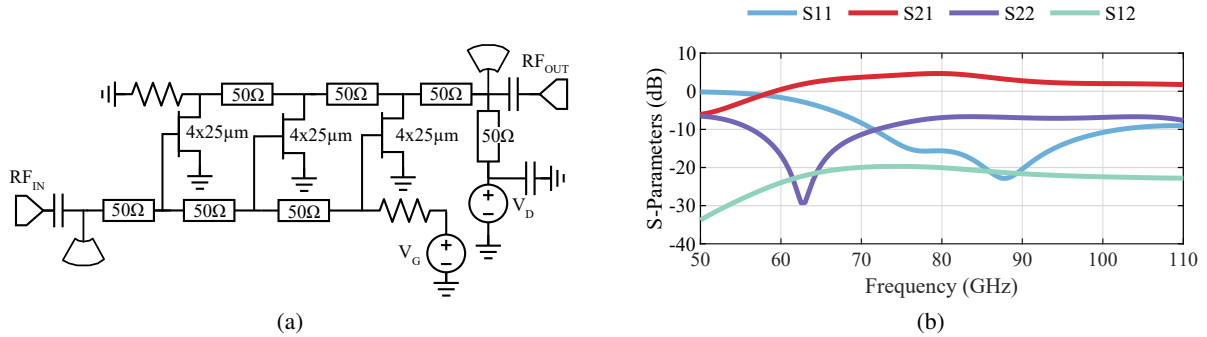
Figure 6.2: (a) Simplified schematic of traveling-wave amplifier used for Circulator 1. The three devices have equal peripheries, while the interconnecting transmission lines have the same impedances but different electrical lengths. (b) Simulated S -parameters of unit distributed amplifier.
