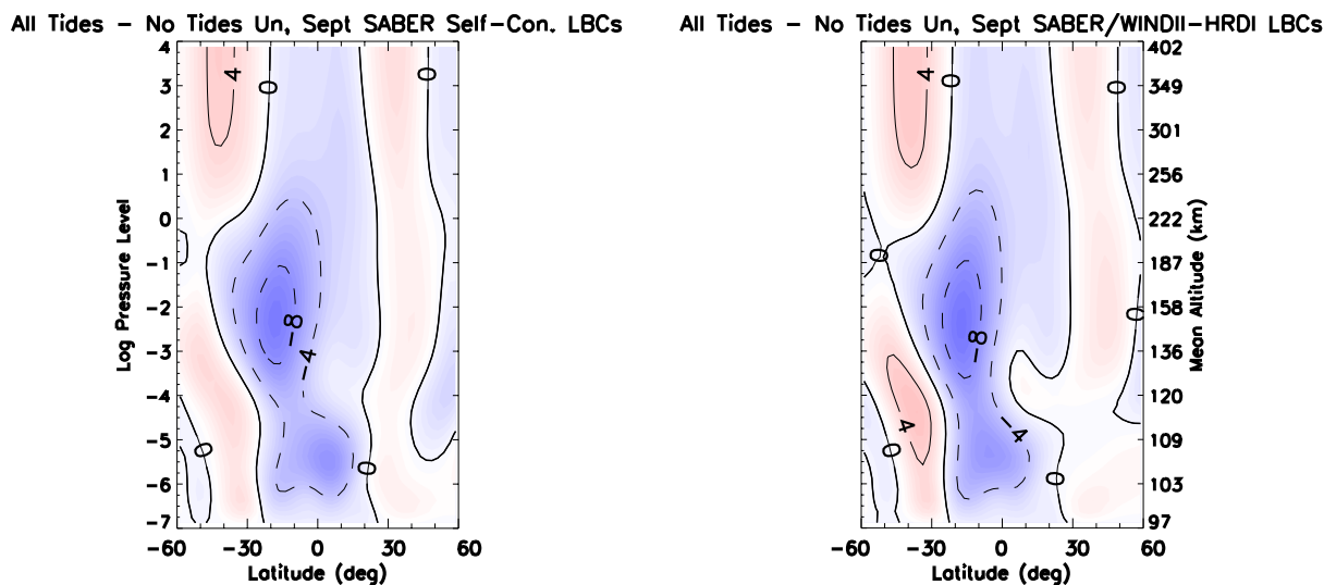
Figure 2.7: TIE-GCM zonally- and diurnally-averaged zonal wind differences as a function of latitude and log-pressure level during the month of September. Differences are calculated between TIE-GCM simulations including and excluding CTMT tidal forcing at the model lower boundary; differences calculated using background winds, temperatures, and geopotential heights from SABER are shown in the left panel; differences calculated using background winds from WINDII-HRDI and background temperatures and geopotential heights from SABER are shown in the right right. Zonal wind differences are contoured every 4 \text{ m s}^{-1} .
