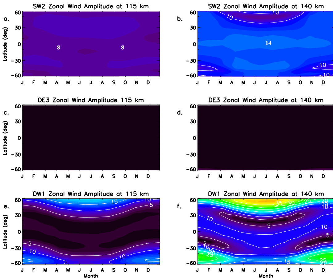
Figure C.1: Same as Figure 4.3, except for TIE-GCM simulations that exclude CTMT lower boundary tidal forcing.
