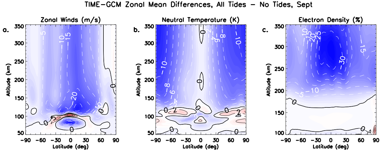
Figure 1.2: September zonally- and diurnally-averaged zonal wind (a), temperature (b), and electron density (c) differences between simulations from the TIME-GCM including and excluding lower boundary tidal forcing for solar minimum conditions.
