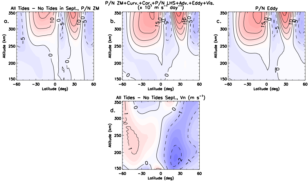
Figure 4.16: TIE-GCM forcing term differences between simulations including and excluding CTMT tidal lower boundary forcing under September and solar medium conditions as a function of latitude and between 150 and 350 km. The P/N ZM term is shown in (a); P/N ZM + Curv. + Cor. + P/N LHS + Adv. + Eddy + Vis. terms in (b); the P/N Eddy term in (c); the zonally-averaged meridional wind differences are shown in (d). Forcing terms from the zonal-mean zonal momentum equation are contoured every \pm 5 \times 10^1 \text{ m s}^{-1} \text{ day}^{-1} , while the zonally-averaged meridional wind differences are contoured every \pm 1 \text{ m s}^{-1} .
