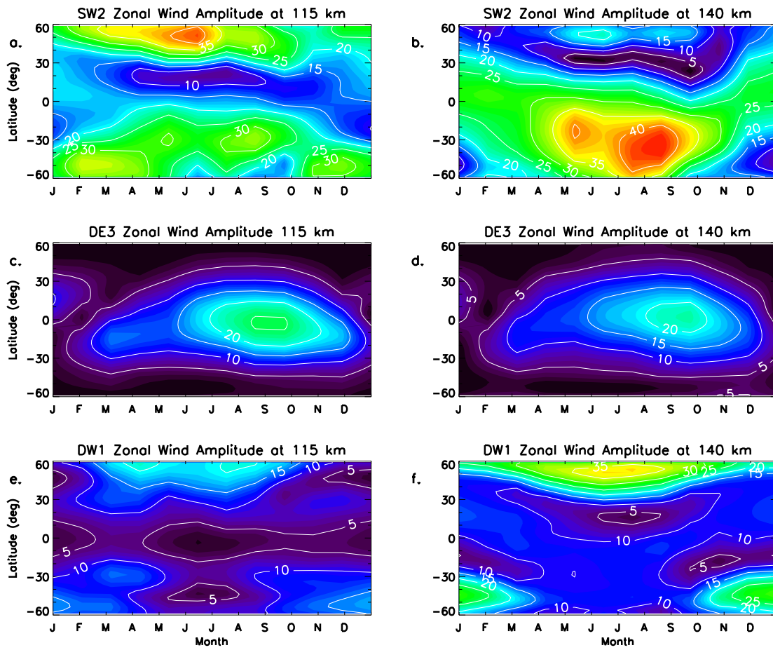
Figure C.8: Same as Figure 4.3, except for a TIE-GCM simulations under solar minimum conditions.
