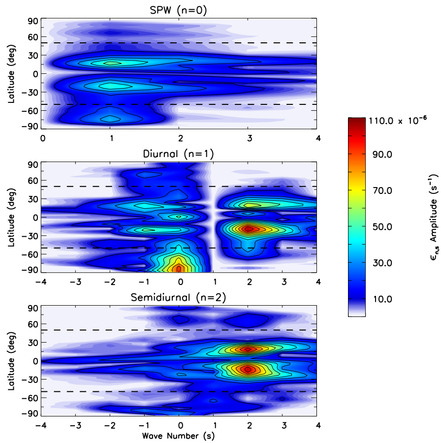
Figure B.5: Same as Figure 3.3, except for the modified flow during solar minimum conditions ( \sim 350 km). Components are contoured every 10 \times 10^{-6} \text{ s}^{-1} .
