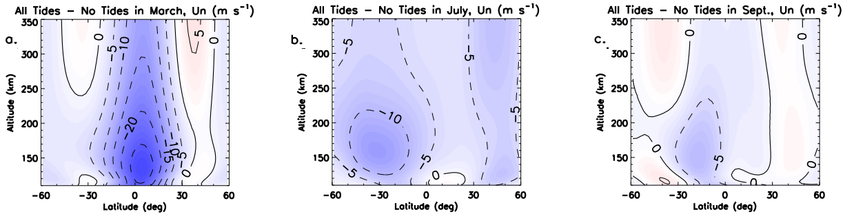
Figure 4.8: TIE-GCM zonal-mean zonal wind differences as function of latitude and altitude during March (a), July (b), and September (c), under solar medium conditions. Zonal mean zonal wind differences are contoured every \pm 5 \text{ m s}^{-1} .
