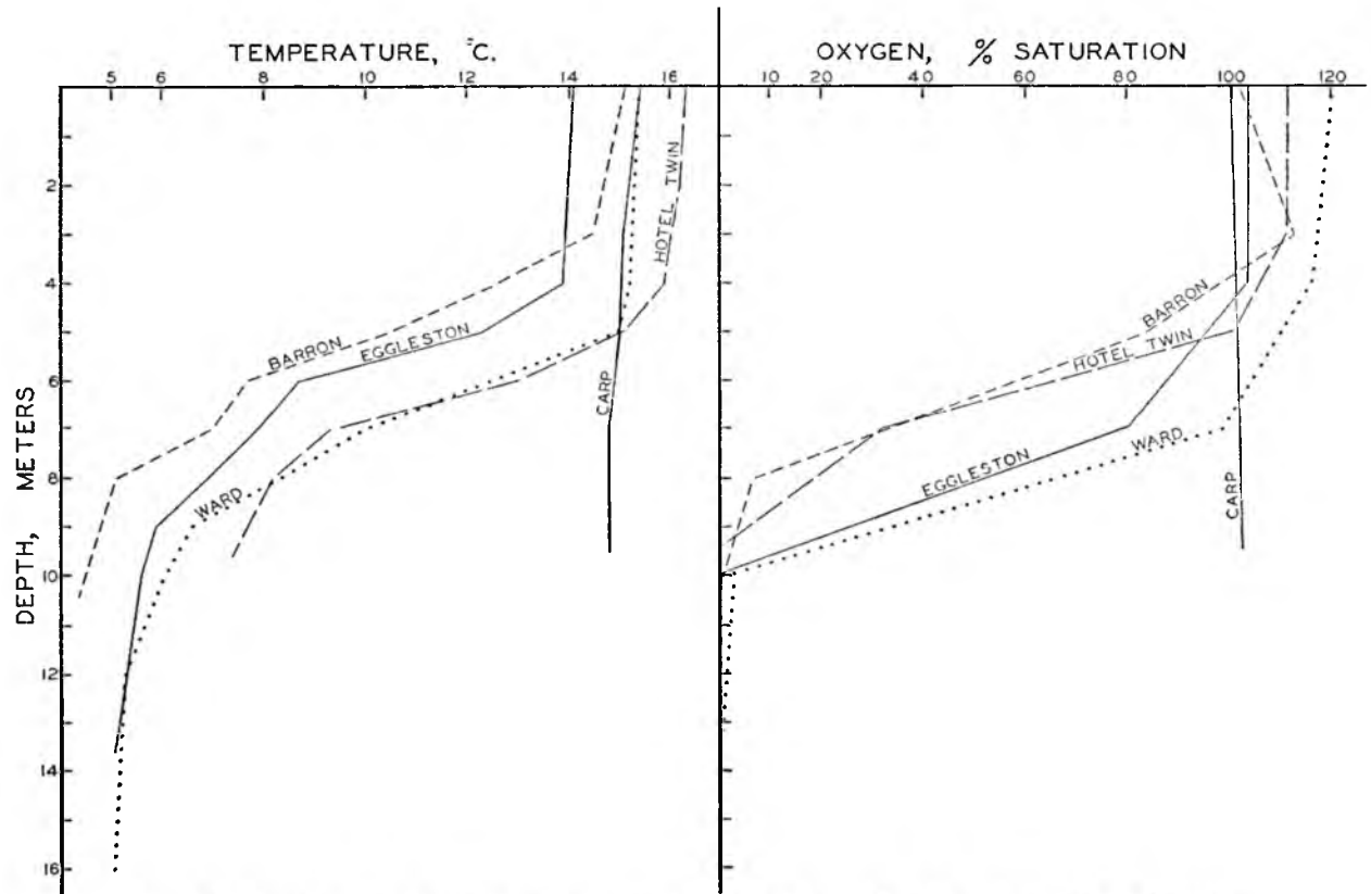
FIGURE 2. Temperature and oxygen stratification curves for five Grand Mesa lakes, August 20 to 25, 1947.
