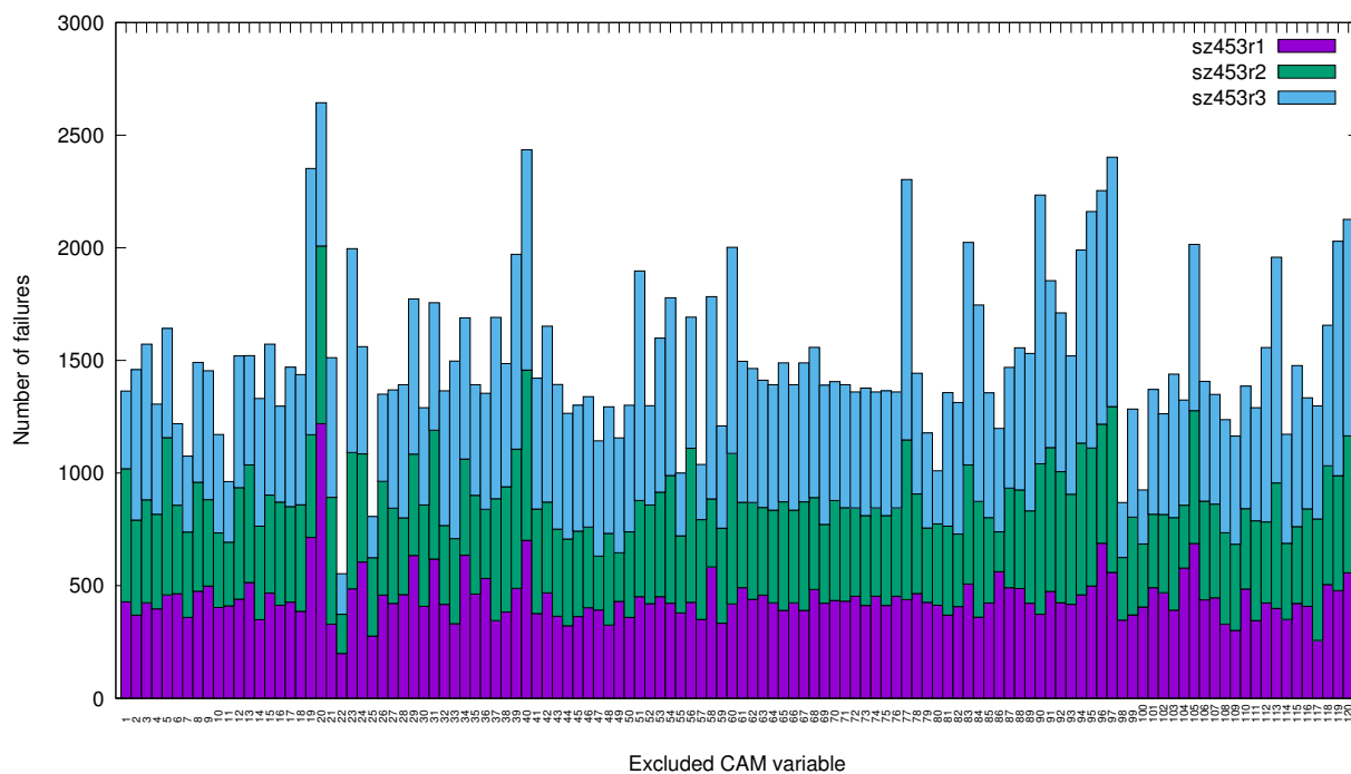
Figure 7.2: Stacked histogram of Mira failures against the three sz453 summary files, with the excluded CAM variable indicated on the x-axis. Note that the number of failures is out of 6072 possible failures.
