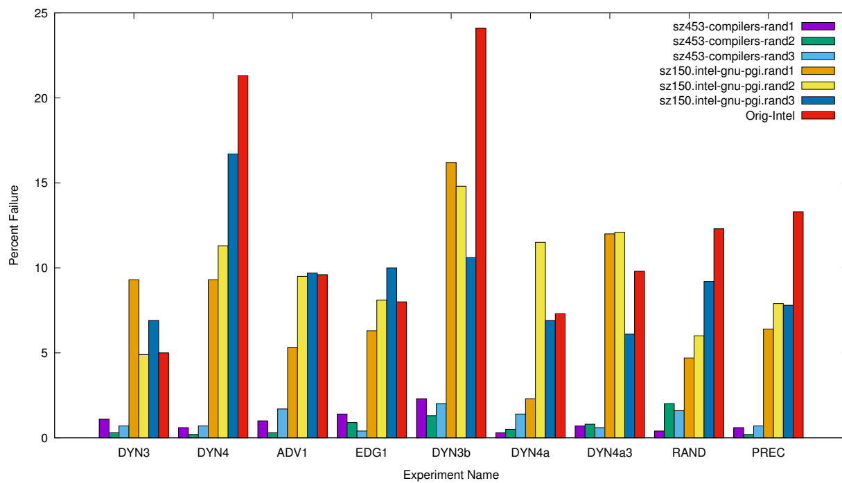
Figure 5.1: Note that the size 453 failure rates are on the order of our desired false positive rate. The CESM-ECT ensemble from BH2015 is featured (Orig-Intel) for comparison with the compiler aggregate rand summaries.
