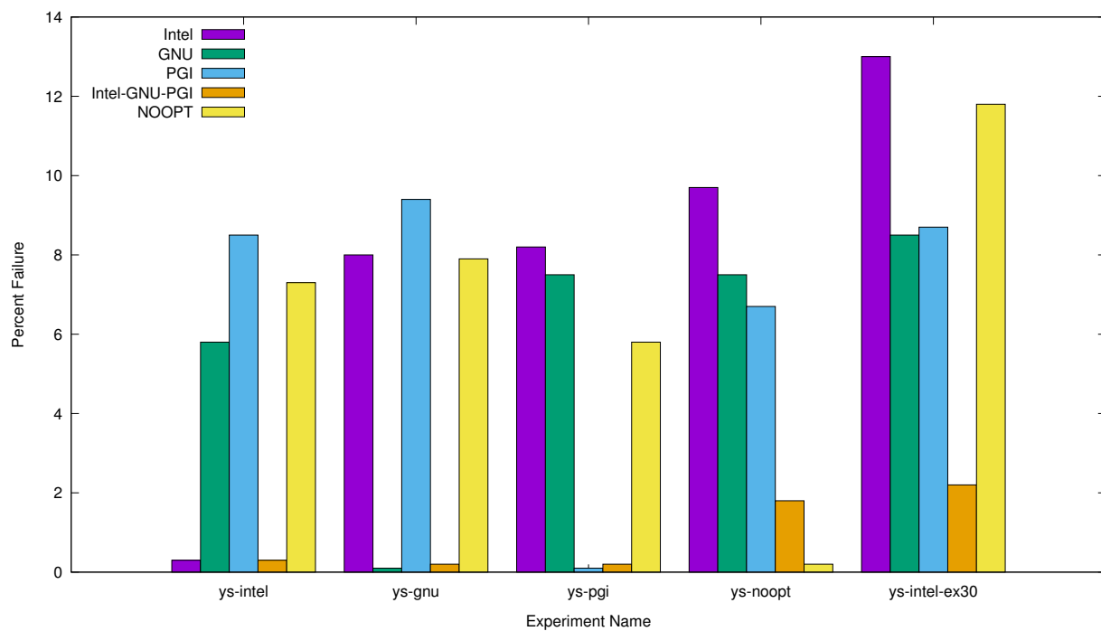
Figure 4.1: EET failure percentage grouped by experiment. Colors indicate ensemble summary file used in comparison, “ys” abbreviates Yellowstone. “Intel” is the CESM-ECT accepted ensemble in BH2015.
