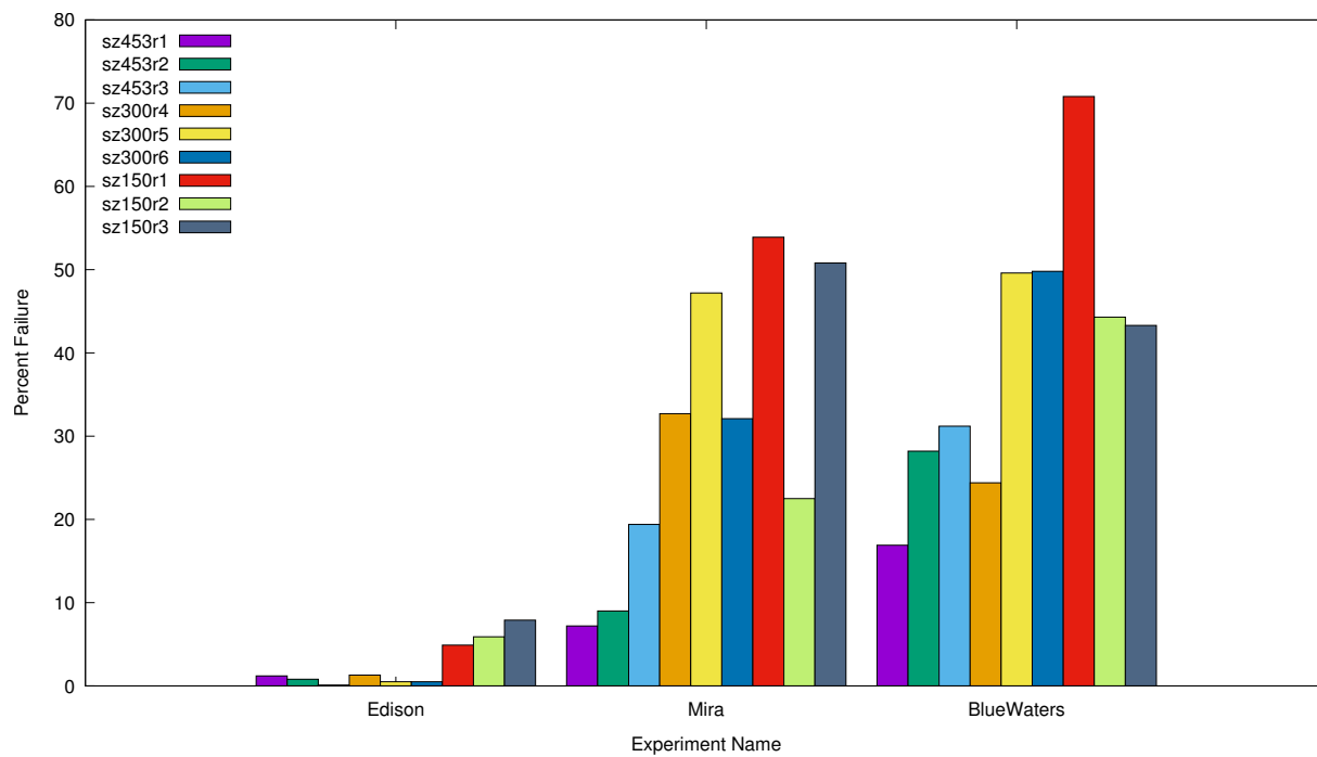
Figure 7.1: Exhaustive testing failure rates of three CESM-supported supercomputers. Mira and Blue Waters were borderline failures using CESM-ECT (see Table 2.3).
