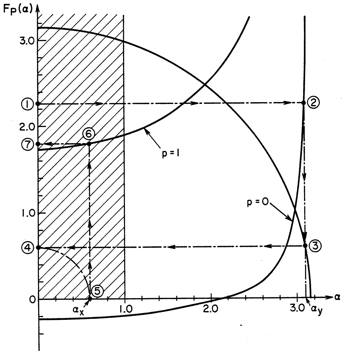
Fig. 6. Characteristic function F_p(\alpha) for a microstrip patch \epsilon_r = 10 , d = 1.27 mm and f = 8 GHz.
