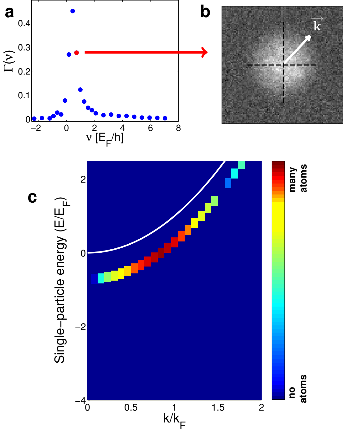
Figure 5.5: Creating the PES plots. a. A line shape showing the relative fraction of atoms outcoupled at each rf detuning. The line shape is normalized such that \int_{-\infty}^{\infty} \Gamma(\nu) d\nu = 1/2 , due to the 50% – 50% spin mixture. b. An image of an atom cloud, taking for the detuning marked in red on the line shape ( \nu \approx 6.5 kHz). In our analysis, this image will be averaged with 2 others at the same detuning, and the momentum distribution will be extracted from the atoms' TOF positions. c. The contribution of a single image to a full PES dispersion plot. The image in b is shown after extracting the momentum distribution. The color corresponds to the fraction of the atoms having a specific momentum. Each frequency on the line shape ( a ) will add a parabolic strip of dispersion data to the plot. Each strip is shifted from the bare transition (the white line, also called the free-particle line) by -\hbar\nu .
