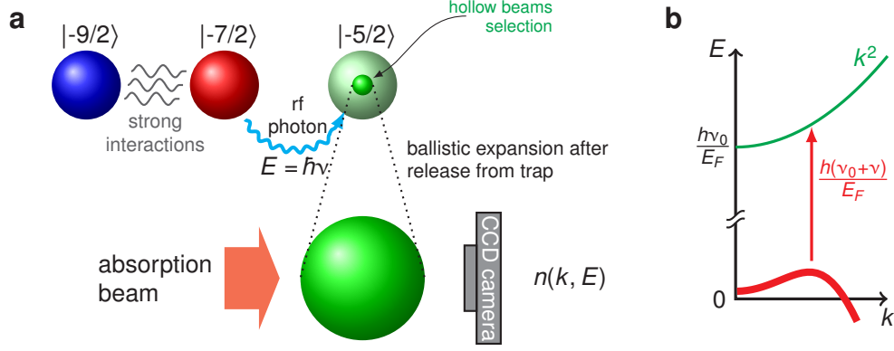
Figure 5.2: Atom photoemission spectroscopy (PES). a. In our PES experiments, we start with an equal mixture of atoms in the |9/2, -9/2\rangle and |9/2, -7/2\rangle states, with a Fano-Feshbach resonance controlling their interactions. An rf photon moves some atoms from the |9/2, -7/2\rangle state to the |9/2, -5/2\rangle state, which does not interact with the first two states. Nearly simultaneously with the rf pulse, the hollow light beams are pulsed and the trapping potential is turned off. The atoms expand and fall during time of flight, and we take an image of only those atoms selected by the hollow beams. b. The signal that we measure from PES is constructed through energy and momentum conservation. By measuring the momentum of the outcoupled atoms (green line), we know the momentum of the atoms in the trap, and we can use the rf photon energy to also get the energy of the atoms in the trap (red line). The shape of the measured dispersion (red line) tells us something about the state of the interacting system (the back-bending seen here can be indicative of BCS-like pairing).
