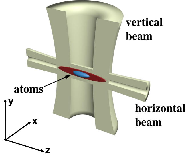
Figure 2.2: Illustration of the two intersecting hollow light beams used to optically pump atoms at the edges of the trapped atom cloud.
