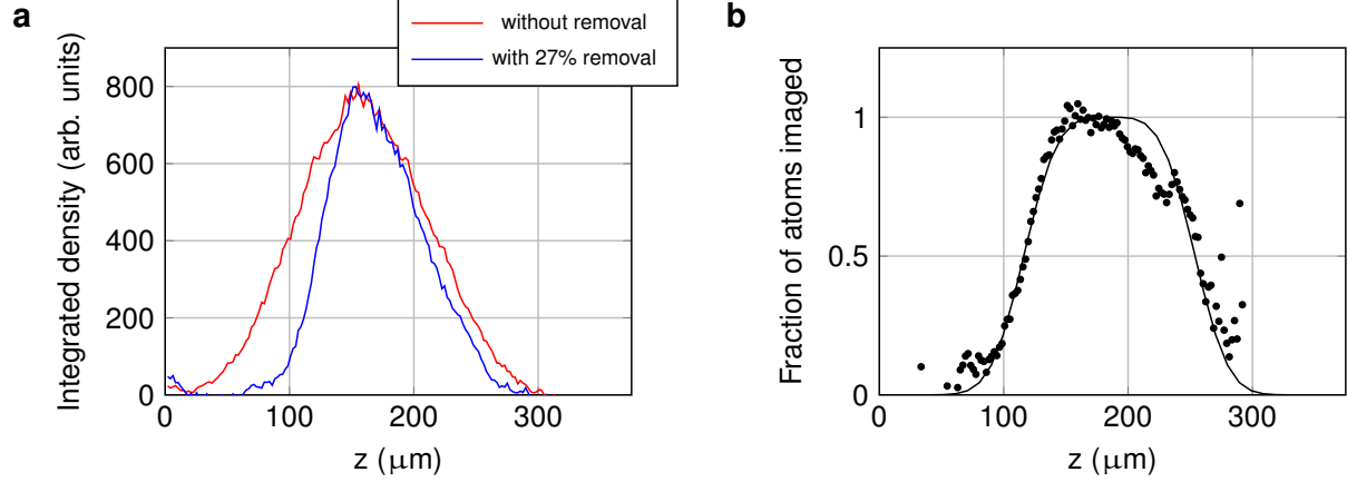
Figure 2.9: The removal of signal by the vertical donut beam. a. Density profiles before and after application of the vertical donut beam. Note that the number of atoms imaged in the center is unchanged, with signal only being removed from the cloud's edges. This shows good alignment of the donut beam onto the atoms. b. The fraction atoms remaining in the signal is shown as a function of z (dots). This is compared to a very simple model predicting the amount of removal from an l = 2 LG beam with a waist of 186 \mu\text{m} (black solid line). This model fits the data well. The slight asymmetry in the removal seen on the upper right side of the data comes from a slight asymmetry in the donut beam profile itself, just visible in figure 2.8b. This is further evidence that the cross section fit by a 186 \mu\text{m} waist corresponds to the correct intensity profile seen by our atoms.
