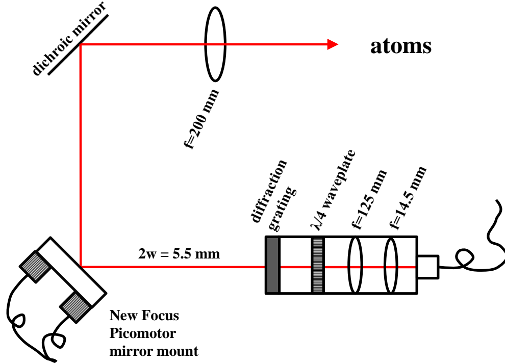
Figure 2.3: Setup of the horizontal donut beam. The horizontal donut-mode beam (propagating along the z -direction) is collimated to a 5.5 mm diameter before it is sent through a forked diffraction grating that gives the beam an l = 2 Laguerre-Gaussian mode in the far field.
