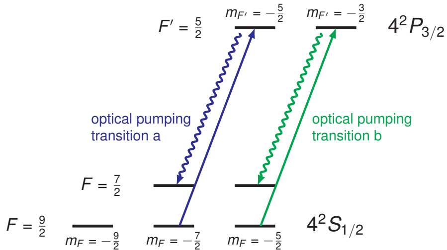
Figure 2.4: Optical pumping transitions. The straight lines indicate the two optical pumping transitions used in the donut beam technique. The squiggly lines indicate the most likely spontaneous decay path of an optically pumped atom.
