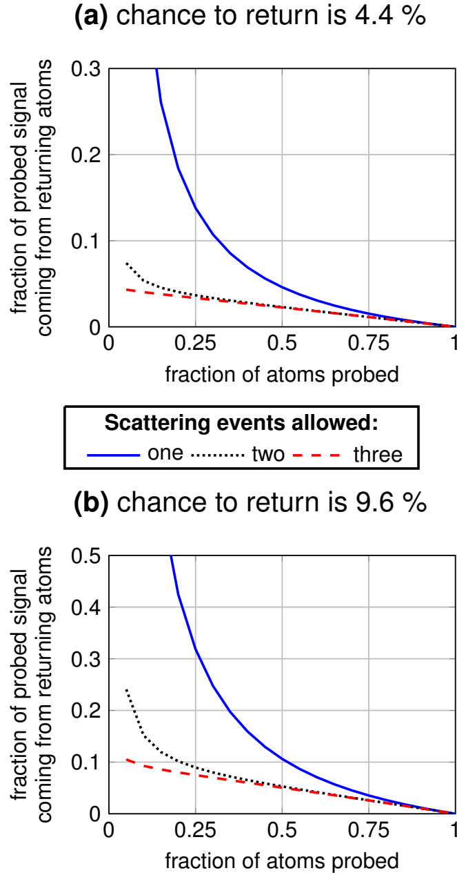
Figure 3.8: The size of the “bad signal” for two branching ratios. Using equation 3.4, I can estimate the fraction of the signal that comes from atoms with an extra momentum kick from having scattered a photon. The blue line is the estimated fraction of bad signal if the atoms can scatter at most one photon. As we account for more scattering events, the atoms which have fallen back into the imaging state after being pumped have another chance to be removed, and the fraction of bad signal begins to converge to a lower value. The two graphs correspond to the two optical pumping transitions we use, found in figure 2.4. From these calculations, we estimate the error from “hot atoms” to be below 5% for transition a and below 10% for transition b .
