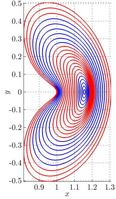
Figure 3.3: L_2 planar periodic orbits
