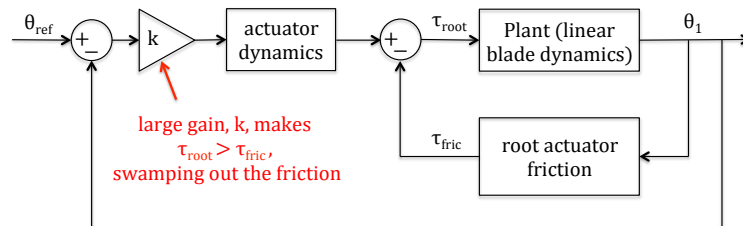
Figure 3.7: Swamping out friction with high gains
