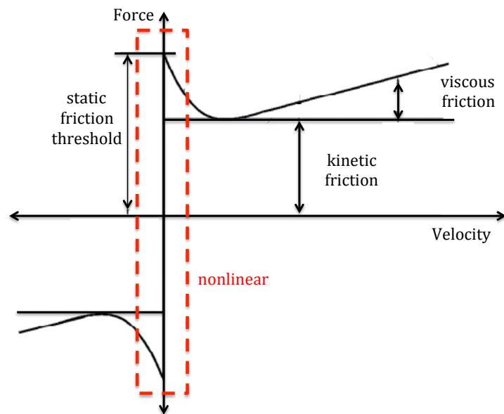
Figure 3.8: Nonlinear friction [13]
