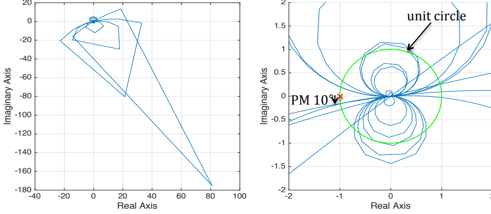
Figure 3.18: Compensated outer loop gain
