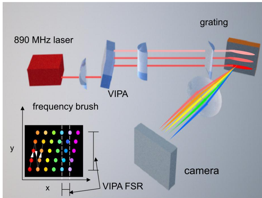
Figure 4.11: The high resolution 2-D setup resolves individual comb lines spaced by 890.4 \text{ MHz} . The VIPA with a FSR of 25 \text{ GHz} separates adjacent comb lines in the y direction and the grating separates repeated orders of the VIPA along the x direction. The white arrows show adjacent comb lines with increasing frequency.
