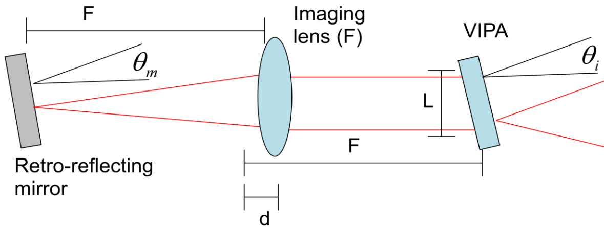
Figure 5.11: VIPA-only pulse shaper dispersion management parameters. Red lines show light focused into the VIPA-only pulse shaper and black lines show dimensions and angles of interest. The input angle of the VIPA, \theta_i , focal length of the imaging lens, F , angle of the retro reflecting mirror, \theta_m , the distance the focusing lens is closer than F to the VIPA, d , and the height of the beam after the VIPA, L all need to be carefully controlled to manage dispersion from the VIPA-only pulse shaper.
