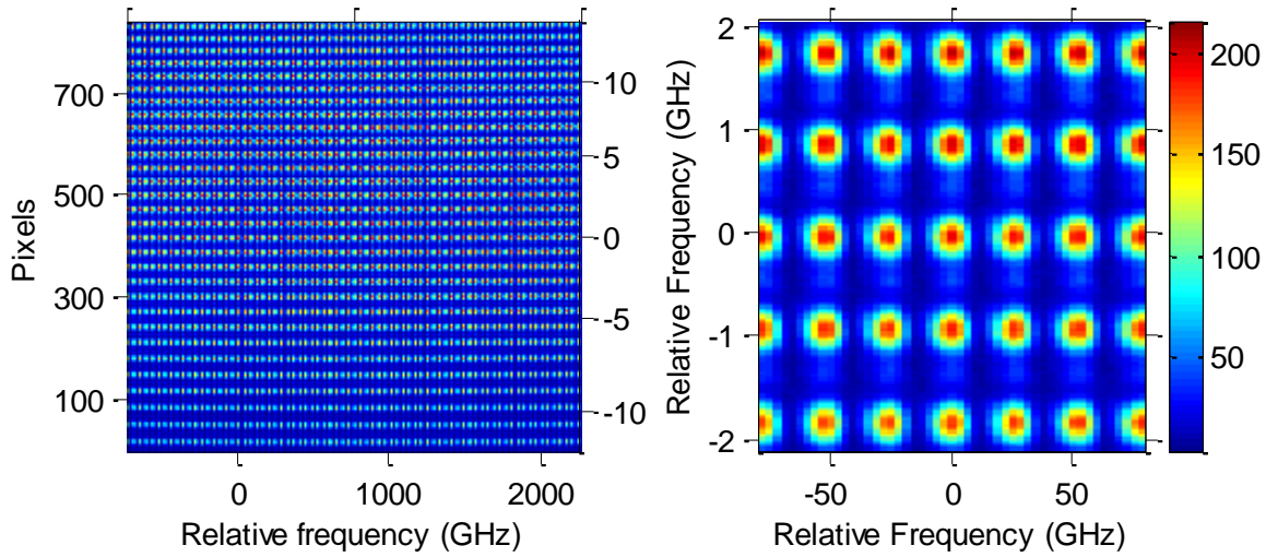
Figure 4.12: Images showing a frequency brush of the resolved discrete frequencies of an 890 MHz pulse train. The image on the left shows the entire VIPA FSR and the image on the right shows a zoomed-in section of the spectrum.
