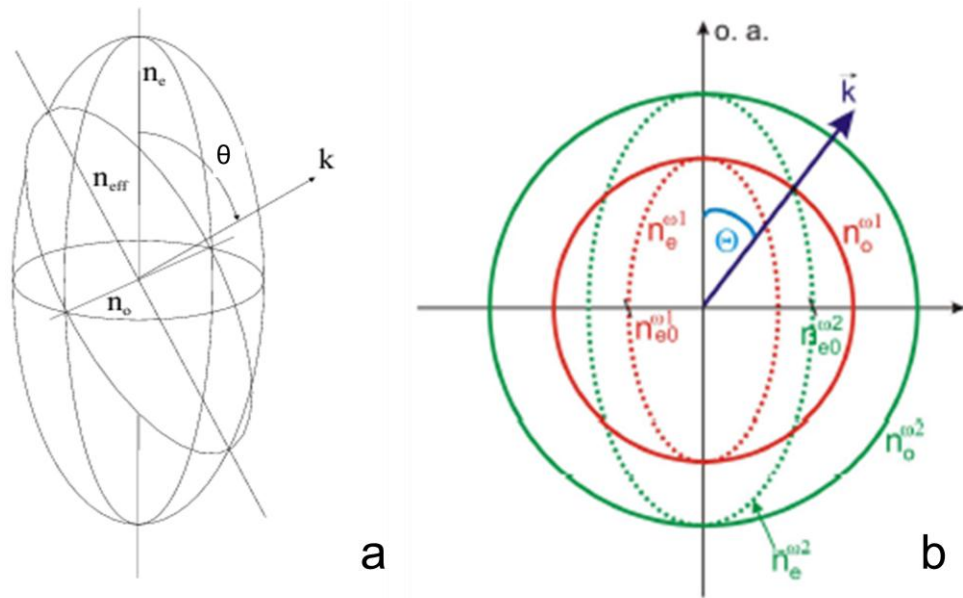
Figure 5.8: Ordinary and Extraordinary index of refraction as a function of angle from the optical axis (a). k-space diagram of ordinary index of refraction at 800 nm ( \omega_1 ) and extraordinary index of refraction at 400 nm ( \omega_2 ), showing necessary angle from optical axis to achieve collinear type I phase matching (b). Images from [42]
