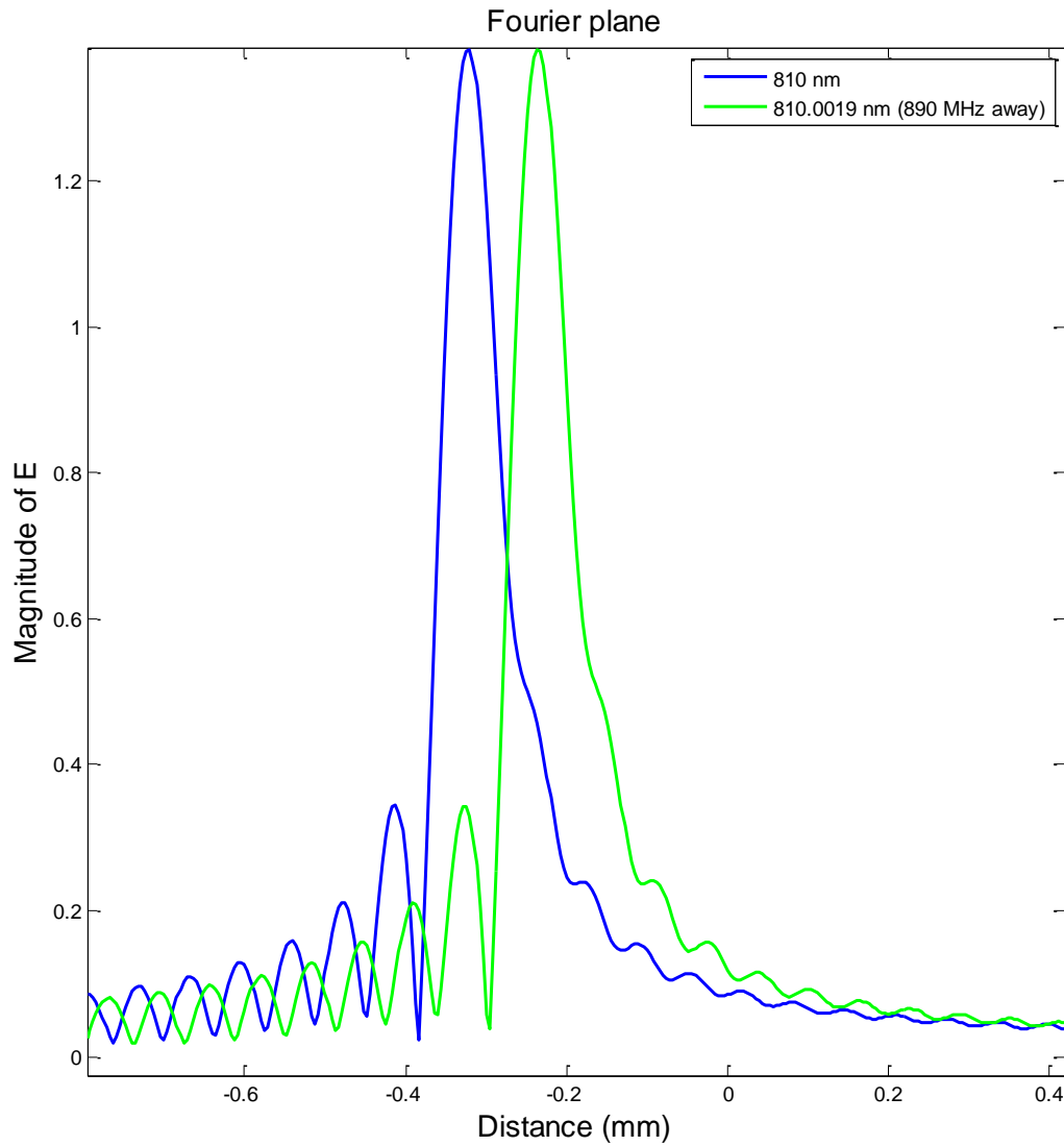
Figure 4.18: Close up of how well resolved the two frequencies are separated from one another in the first order of the VIPA.
