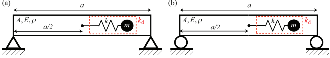
Figure 5.3: Finite rod with an attached spring-mass resonator and (a) fixed-fixed or (b) free-free boundaries.
