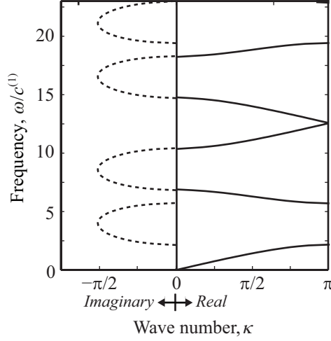
Figure 1.2: Frequency band structure for a 1D phononic crystal. Solid curves represent pass bands, and dashed curves represent stop-bands.
