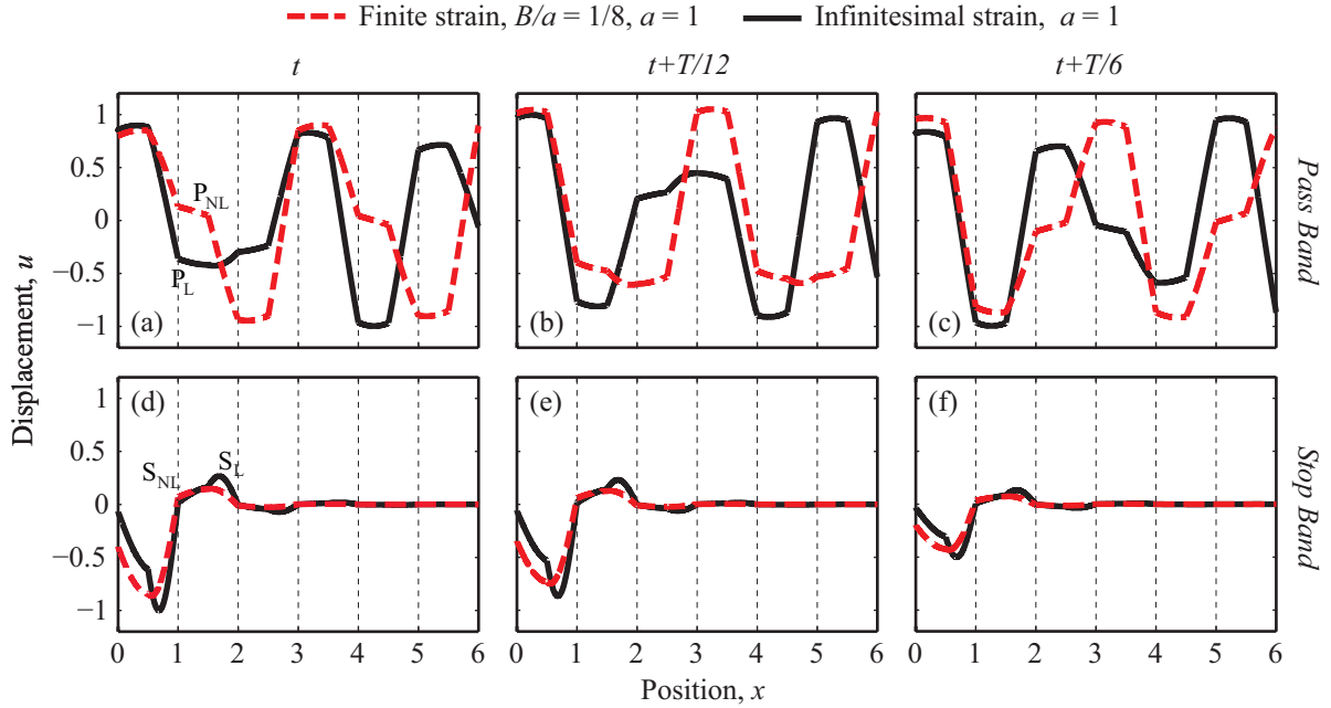
Figure 4.5: Three time snap shots of the Bloch mode shape over six unit cells corresponding to the four points P_L , P_{NL} , S_L , and S_{NL} marked in Fig. 4.3. The Bloch mode shape for points P_L and P_{NL} are shown in (a), (b), and (c), while the Bloch mode shapes for points S_L and S_{NL} are shown in (d), (e), and (f). Red dashed curves correspond to finite strain and black solid curves correspond to infinitesimal strain. Each pass-band and stop-band sets of curves are normalized with respect to the maximum displacement value of the infinitesimal strain case at time t .
