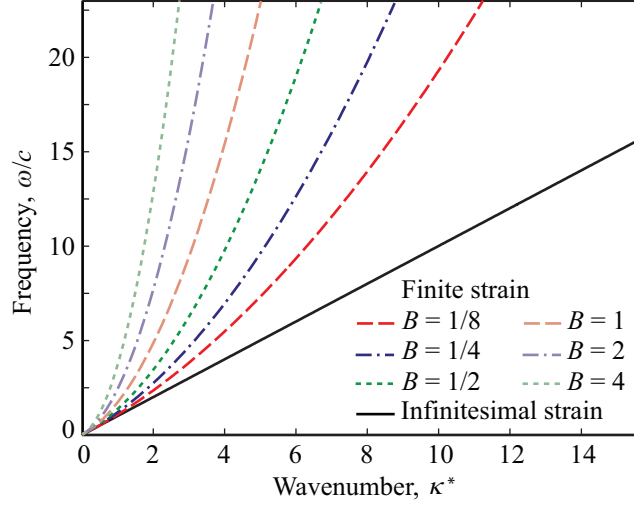
Figure 5.4: Frequency dispersion curves for a 1D homogeneous elastic medium [1]. The finite-strain dispersion relation is based on Eq. (5.58); the infinitesimal strain dispersion relation is based on Eq. (5.59).
