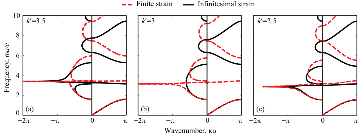
Figure 5.6: Frequency band structure for 1D MM with properties of m' = 3 and (a) k' = 3.5 , (b) k' = 3 , and (c) k' = 2.5 . The results shown are for B' = 1/8 .
