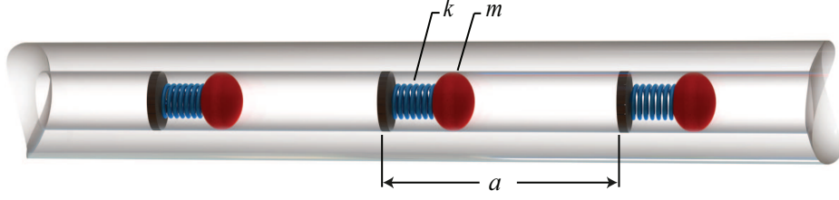
Figure 5.1: A finite section consisting of three unit cells of an infinite 1D nonlinear elastic MM.
