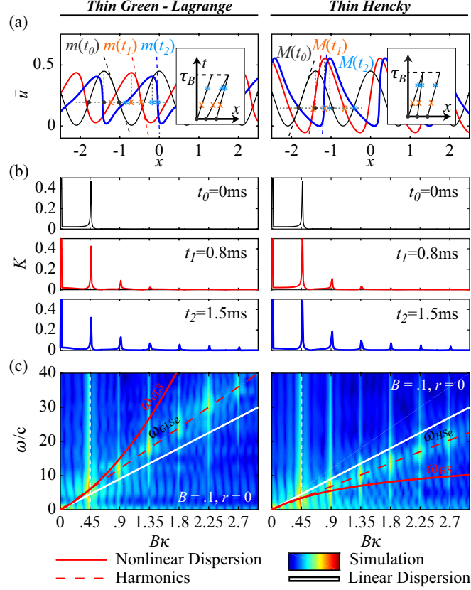
Figure 2.1: (color). Profile snap shots for three different times and their corresponding harmonics. (a) Profiles captured at t_0 = 0 ms, t_1 = .8 ms, and t_2 = 1.5 ms. Inset shows the characteristic lines of the corresponding wave. (b) Normalized distribution of the harmonics generated through time. (c) Wavenumber-frequency spectrum at t_2 represented by the logarithmic spectrum S^2 for the considered value of \kappa_e = 4.5 .
