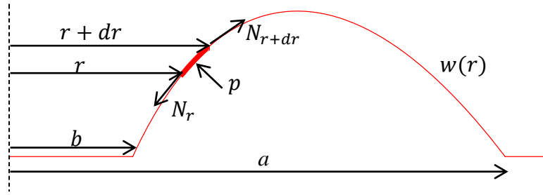
Figure 4.3 Schematic showing a ring element (thicker part of the curve) with the relevant forces
