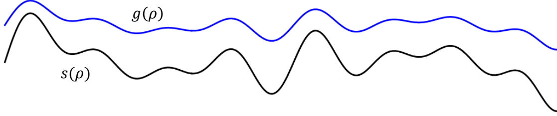
Figure 7.2 Illustration showing the morphology of a graphene membrane (blue) on a corrugated substrate (black)
