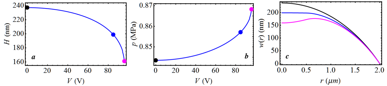
Figure 6.4 Plots showing (a) Central deflection, H and (b) Cavity pressure, p against the applied voltage, V for the geometry with a = 2\text{ }\mu\text{m} , b = 0.5\text{ }\mu\text{m} and h = 500\text{ nm} . The plots in (c) are the deflection profile of the membrane at 0\text{ V} (black), 85\text{ V} (blue) and at pull-in voltage, V_{PI} = 95.9\text{ V} (magenta). These points are highlighted in plots (a) and (b) with the same colors.
