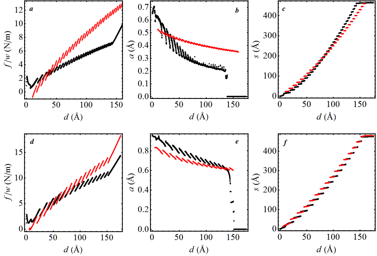
Figure 7.20 (a,d) Force per unit length, (f/w) vs Displacement, d , (b,e) Amplitude, a vs d and (c,f) Crack length, s vs d for \lambda = 15 \text{ \AA} and 30 \text{ \AA} respectively. The data in black and red are from the simulations and theory respectively.
