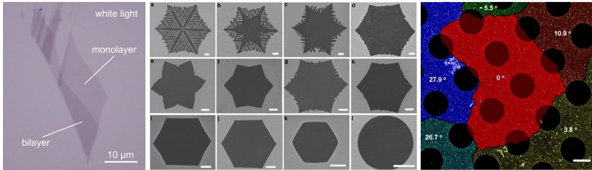
Figure 1.2 (a) Optical image of exfoliated graphene flake on 90 nm SiO 2 (from grapheneindustries.com) (b) Scanning electron microscopy (SEM) images of single crystal CVD graphene of various shapes grown on liquid Cu under different conditions 15 (all scale bars – 5 μm) (c) Scanning transmission electron microscopy (STEM) image of a polycrystalline CVD graphene flake with grains and grain boundaries identified 16 (false colors, scale bar – 1 μm)
