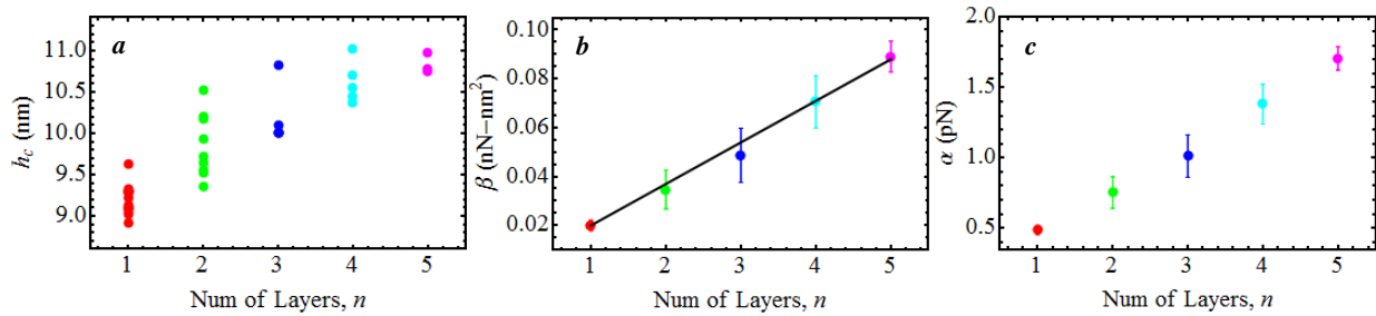
Figure 5.7 (a) Pull in distance, h_c , vs. number of layers for devices with 2a = 3.0 \mu\text{m} and 2b = 0.50 \mu\text{m} . (b) The calculated values of \beta vs. number of layers using the data in (a) assuming p_{att} = \beta/h^4 and S_0 = 0.07 N/m. A best fit line through the data is also shown which has a slope of 0.017 nN-nm 2 /layer. (c) The calculated values of \alpha vs. number of layers using the data in (a) assuming p_{att} = \alpha/h^2 and S_0 = 0.07 N/m.
