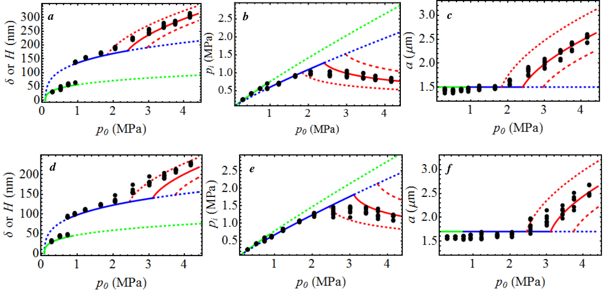
Figure 4.18 (a, d) Maximum deflection ( \delta = \text{spherical} , H = \text{annular} ); (b, e) equilibrium pressure in the microcavity ( p_i ); and (c, f) outer radius of the circular bulge ( a ) versus the charging pressure ( p_0 ). Figures (a,b,c) are for graphene monolayers and (d,e,f) are for multilayers. In each case the symbols are measurements and the curves are theory. The green curve is for the annular deformation, the blue curve for the spherical deformation without delamination, and the red curves are for spherical deformation with delamination for different values of adhesion energies: dashed – 100 (120) \text{mJ/m}^2 , solid – 140 (160) \text{mJ/m}^2 and long dashed – 180 (200) \text{mJ/m}^2 for monolayer (multilayer) membranes.
