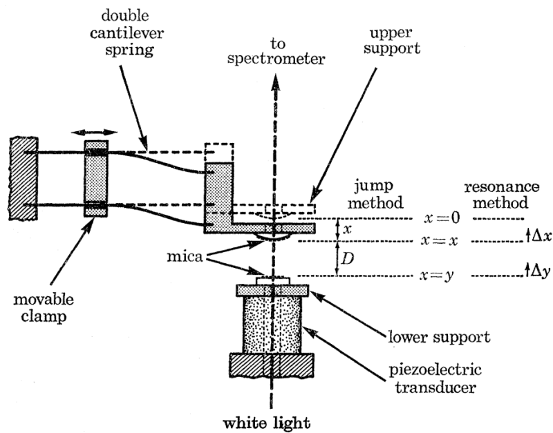
Figure 2.3 Schematic of the surface forces apparatus 67
