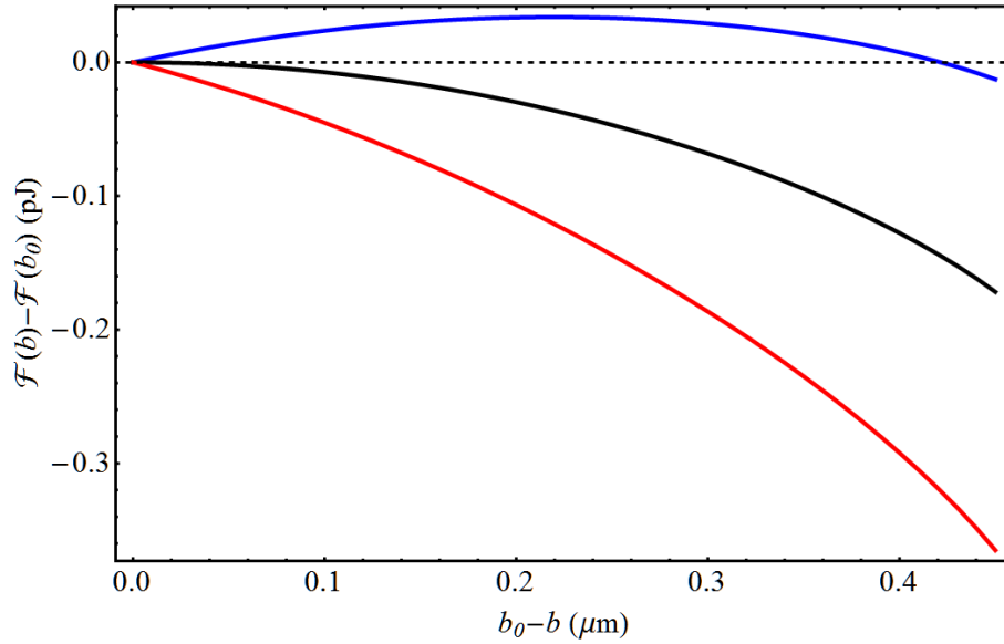
Figure 4.7 Plots showing the free energy variation at fixed a = a_0 as a function of the difference of initial inner radius and inner blister radius at different pressures - (blue) p = 0.6 MPa, (black) p = 0.99 MPa = p_{c,b} and (red) p = 1.4 MPa.
