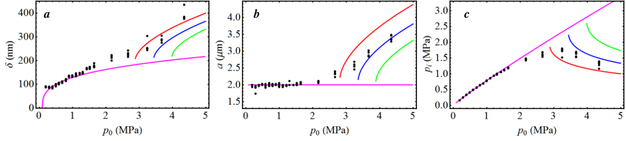
Figure A.5 Plots showing maximum deflection \delta (a), blister radius a (b) and final equilibrium pressure p_i (c) versus input pressure p_0 for all five-layer membranes on Chip A. The magenta colored curve is a theoretical curve assuming no delamination of the membrane for E_t = 1690 \text{ N m}^{-1} , n = 5 . Red, Blue and green curves are theoretical curves for three different values of the graphene/ \text{SiO}_2 adhesion energy \Gamma = 0.24, 0.30, 0.36 \text{ J/m}^2 respectively.
