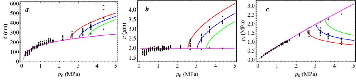
Figure 3.15 Plots showing maximum deflection \delta (a), blister radius a (b) and final equilibrium pressure p_i (c) versus input pressure p_0 for all two-layer membranes studied. The magenta colored curve is the theoretical curve assuming no delamination of the membrane for n\text{Et} = 661 \text{ N m}^{-1} , n = 2 . Red, Blue and green curves are the theoretical curves for three different values of the graphene/SiO 2 adhesion energy \Gamma – 0.25, 0.31, 0.37 J/m 2 respectively.
