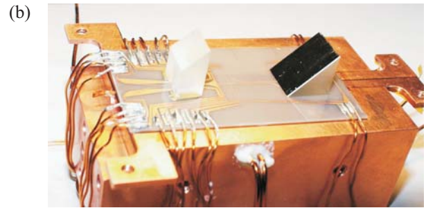
FIG. 1. (a) Schematic drawing of the atom chip (not to scale). The prism-shaped mirrors are integrated with microfabricated wires on an aluminum nitride substrate. The dimensions of the whole chip are 5 cm by 2 cm. (b) A photo image of the atom chip glued onto a copper holder.
